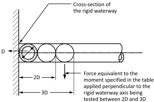
Figure 4 Bending moment on supply fittings (See Clause 5.7.1.2.)
