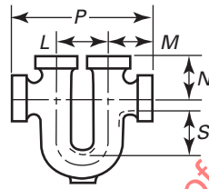
Running Trap Double Vent
