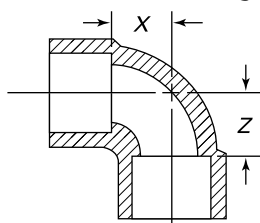
90-deg Elbow C × C
