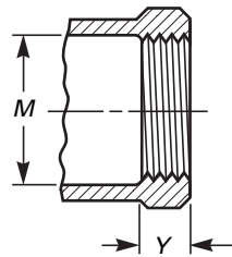
Internal Threaded End (F)
