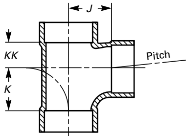
DWV Tees C X C X C
