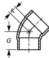
DWV 45 deg FTG Ell FTG X C
