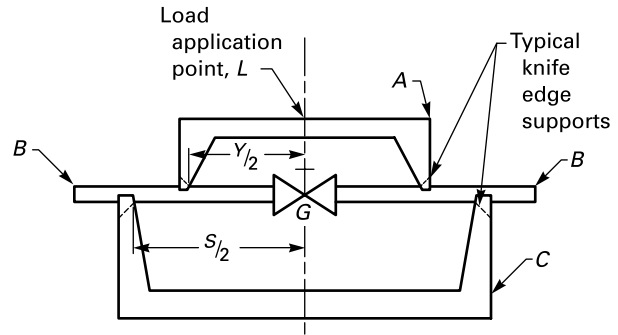
Figure 4.4.4-1 Test Assembly
