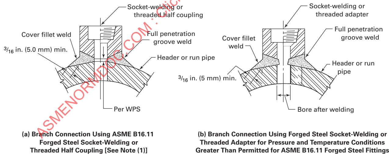
(16) Fig. 127.4.8(F) Typical Full Penetration Weld Branch Connections for NPS 3 (DN 80) and Smaller Half Couplings or Adapters
