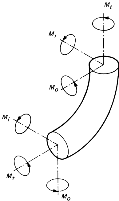
Figure IP-6.1.5-1 Moments in Bends
