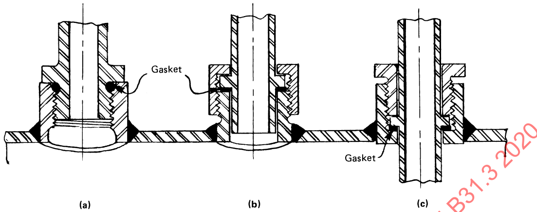
Figure 335.3.3 Typical Threaded Joints Using Straight Threads
