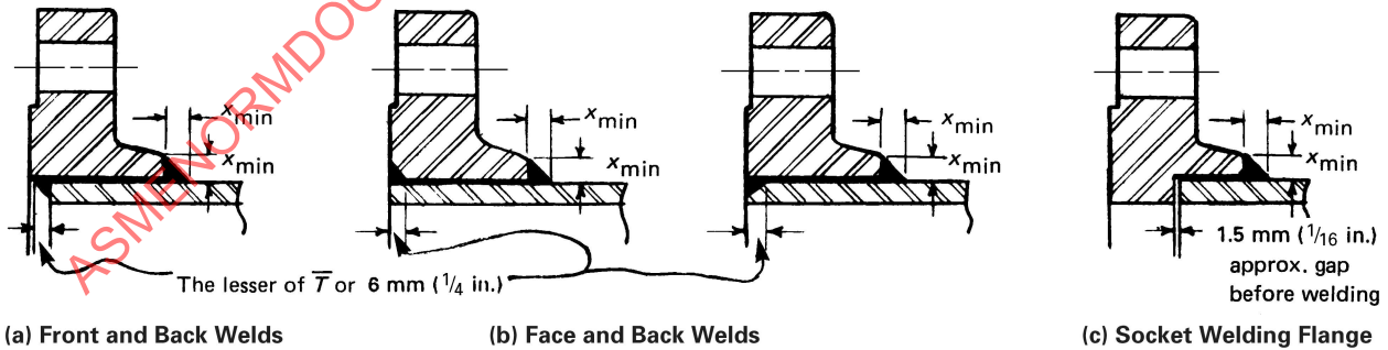
Figure 328.5.2B Minimum Attachment Weld Dimensions for Double-Welded Slip-On and Socket Welding Flanges (20)
