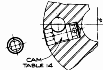
SECTION B-B THRU CAM WITH CAM IN OPEN POSITION
