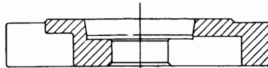
SECTION C-D-E THRU DOG PLATE
