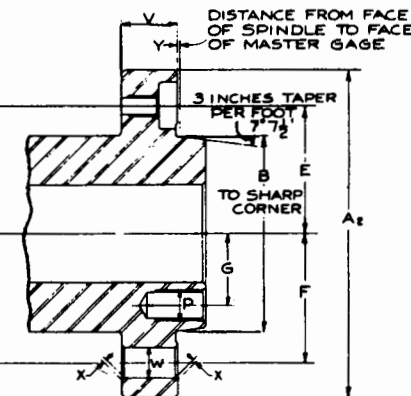
TYPE B SPINDLES
