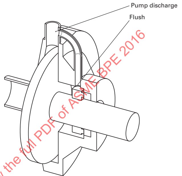
Fig. SG-2.3.2.4-4 Flush Plan 11
