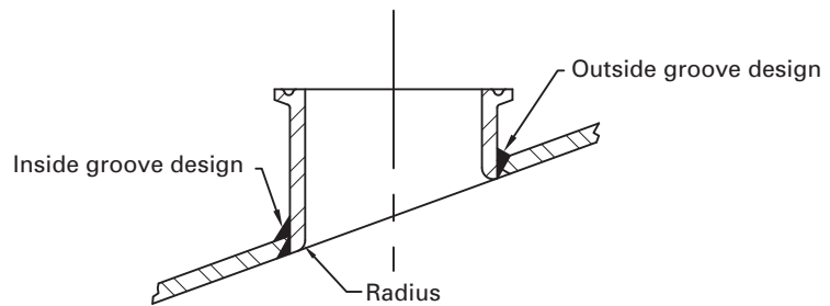
Fig. SD-3.4.2-5 Typical Nozzle Detail
