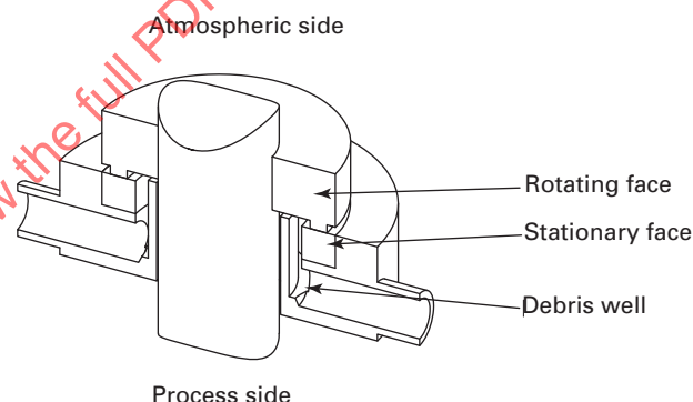
Fig. SG-2.3.2.2-2 Single Seal for Top-Entry Agitator
