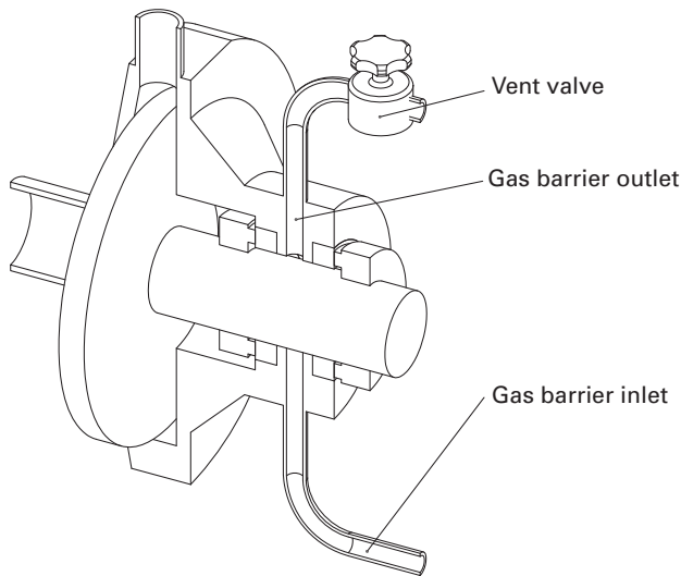
Fig. SG-2.3.2.4-15 Flush Plan 74 for Pump
