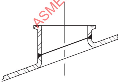
(a) Swage/Butt Weld Design (Accepted: If Vessel Wall Is Thin Enough to Flare)
