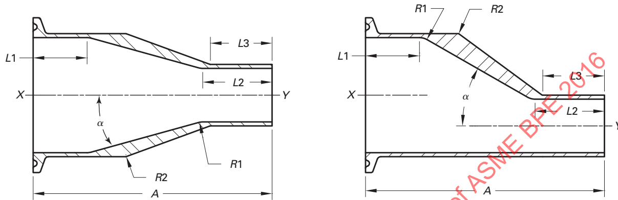
(16) Table DT-4.1.3-2 Hygienic Clamp Joint: Tube Weld Concentric and Eccentric Reducer
