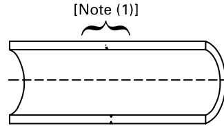
(b) Unacceptable Crack or Crevice on I.D. or O.D.
