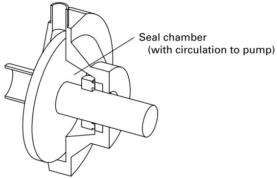
Figure MC-2.3.2.4-3 Plan 03
