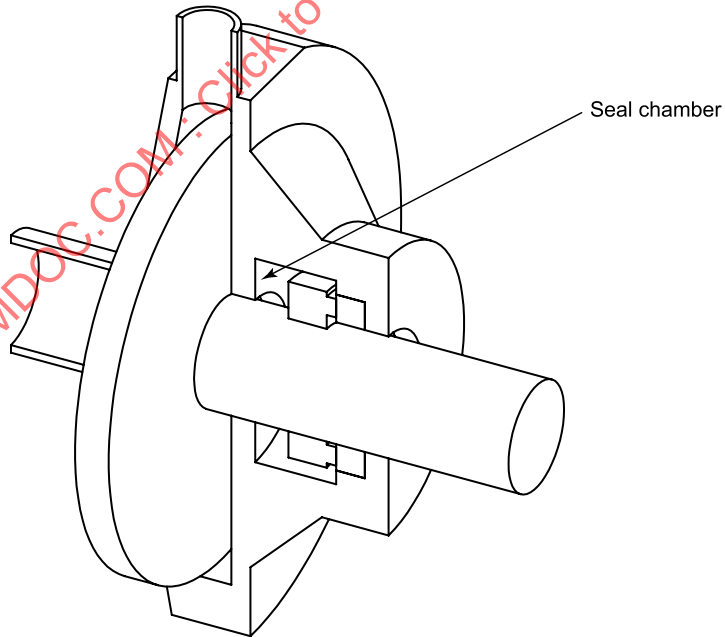
Figure MC-2.3.2.4-2 Plan 02
