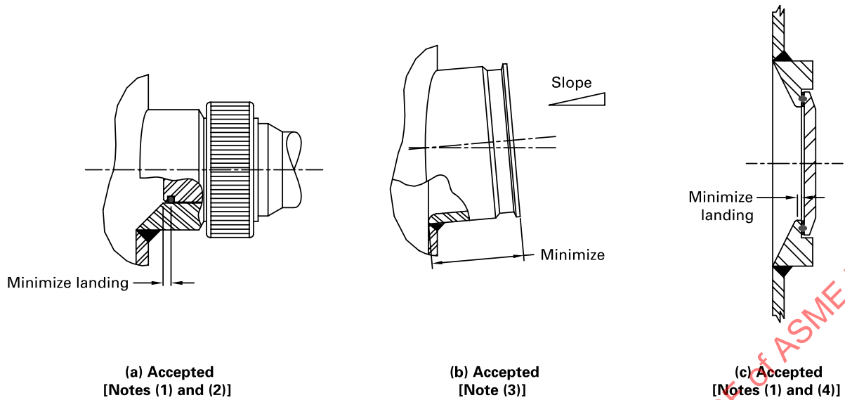
Figure SD-3.4.2-3 Sidewall Nozzles
