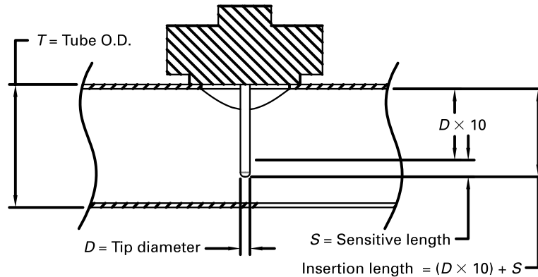
(a) Optimum Insertion Length
