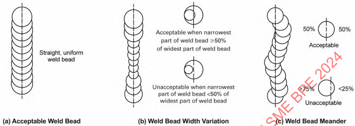
Figure MJ-8.4-4 Acceptable and Unacceptable Metallic Weld Bead Width and Meander on Non-Process Contact Surfaces of Groove Welds on Tube-to-Tube Butt Joints
