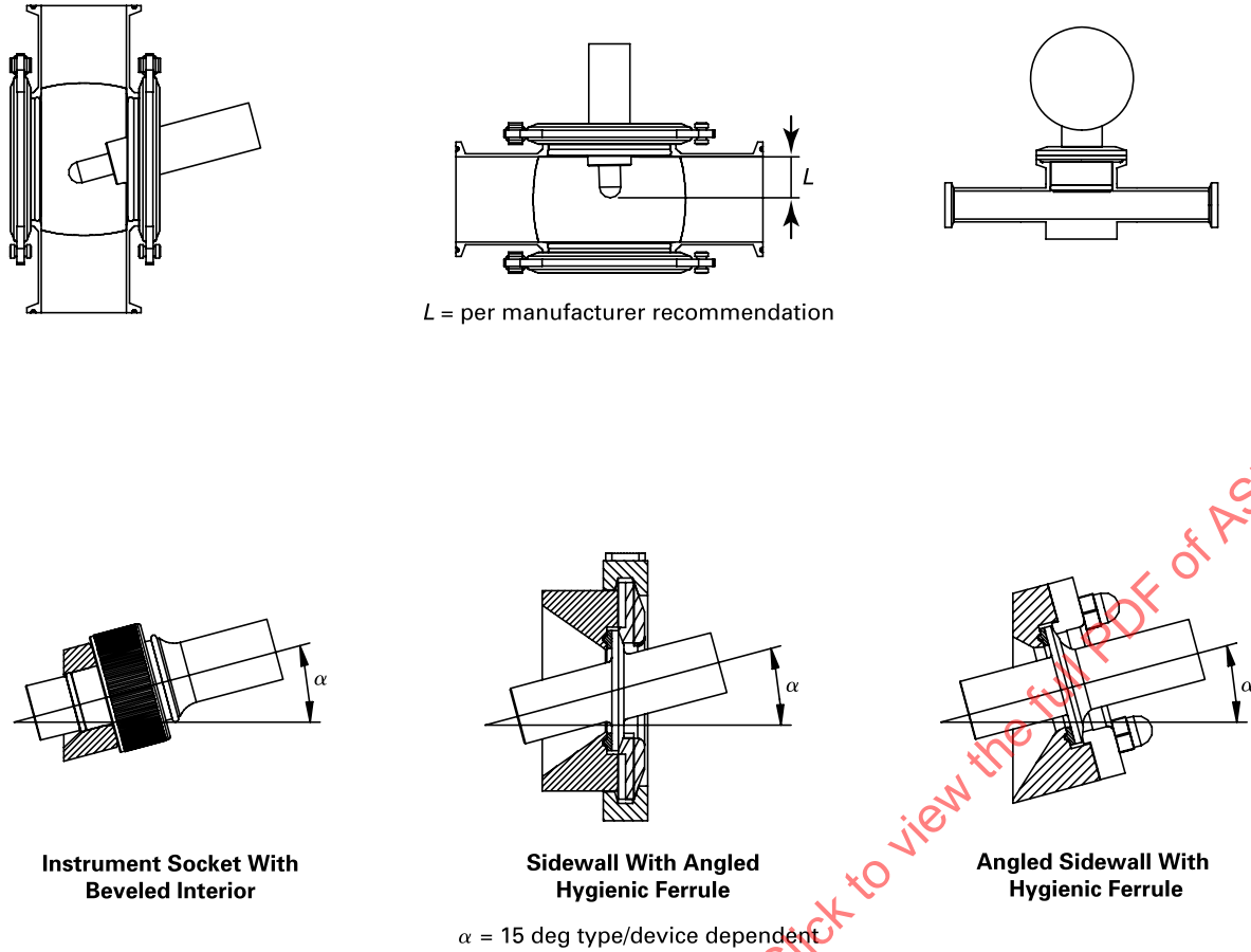
Figure PI-2.2.2-1 Accepted Insertion Device Installation Examples
