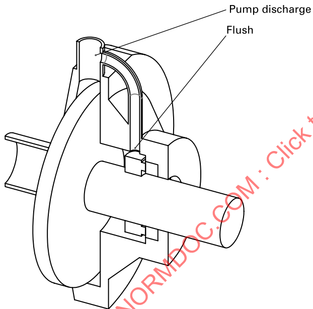
Figure MC-2.3.2.4-4 Plan 11
