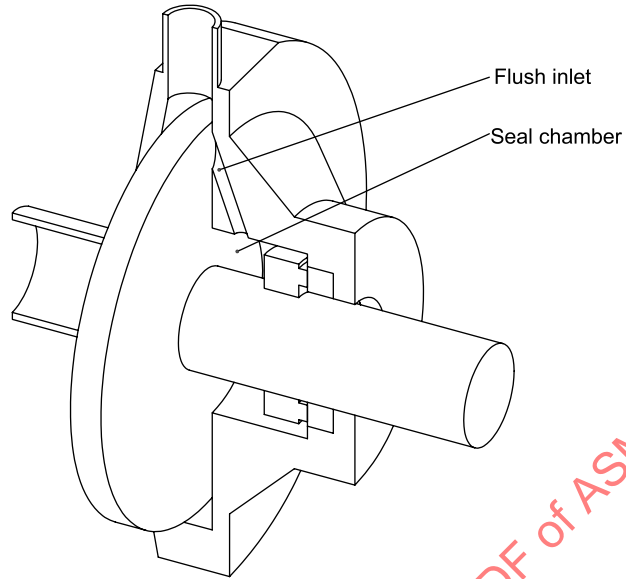
Figure MC-2.3.2.4-1 Plan 01
