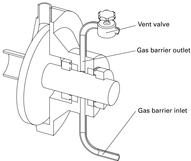
Figure MC-2.3.2.4-15 Plan 74 for Pump
