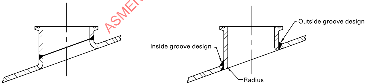
Figure SD-3.4.2-5 Typical Nozzle Detail
