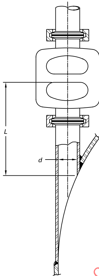
Figure SD-3.4.2-4 Vessel Design Tangential Nozzles
