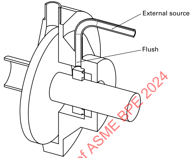
Figure MC-2.3.2.4-5 Plan 32
