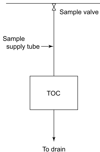
Figure PI-8.4.3-1 Accepted Installation for a TOC Instrument
