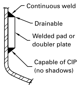
(c) Good Design (Accepted)
