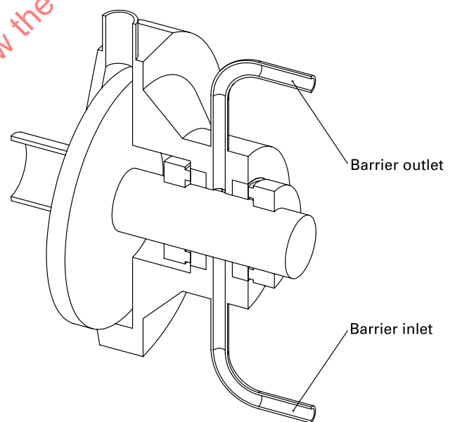
Figure MC-2.3.2.4-10 Plan 54 for Pump
