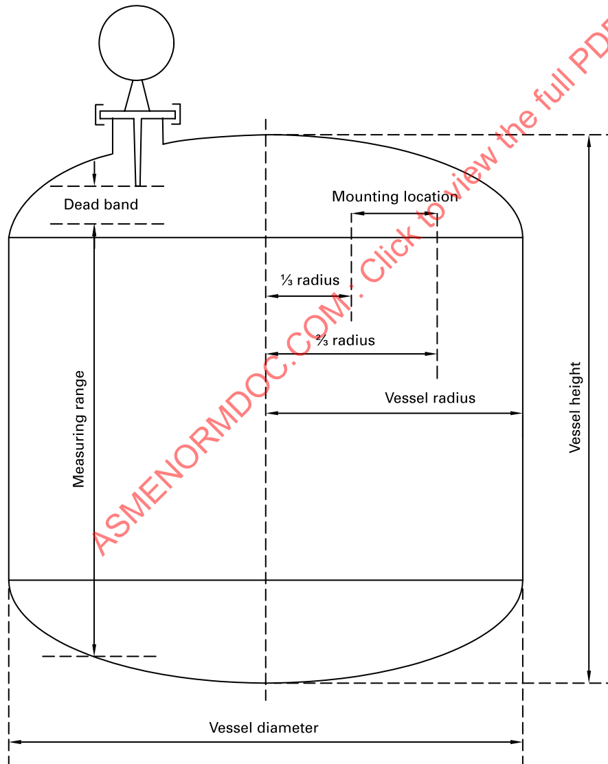
Figure PI-5.1.3.1-1 Dead Band, Measuring Range, and Mounting Location
