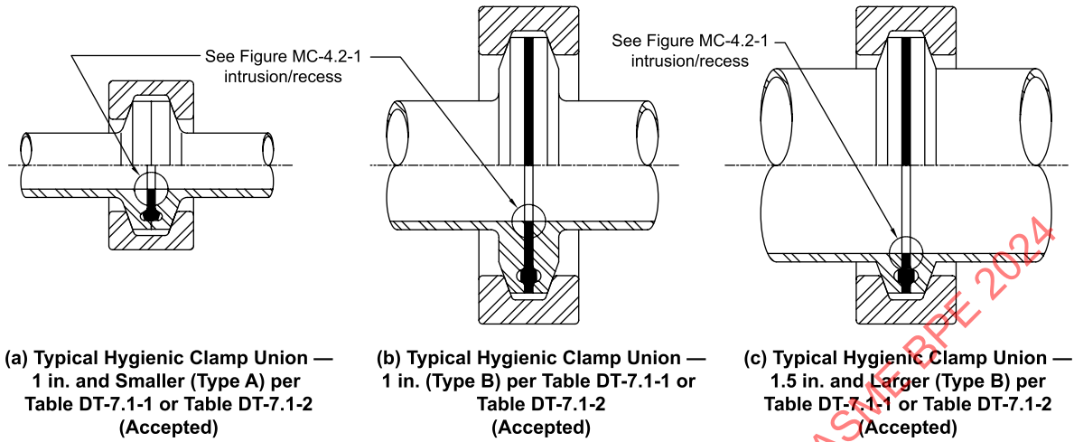
Figure MC-2.2.2-1 Hygienic Union, Ferrules per Table DT-7.1-1 or Table DT-7.1-2
