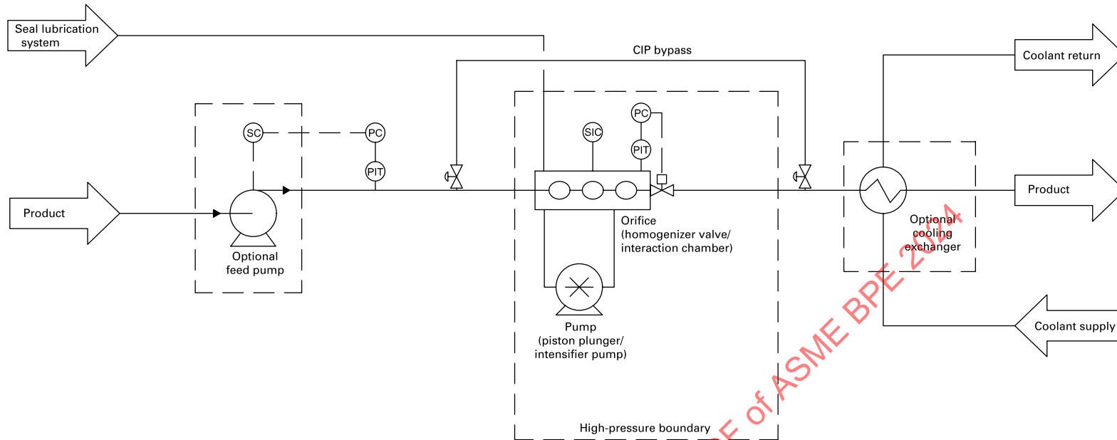
Figure SD-5.2.1-1 Cell Disruptor Process Flow Schematic Diagram
