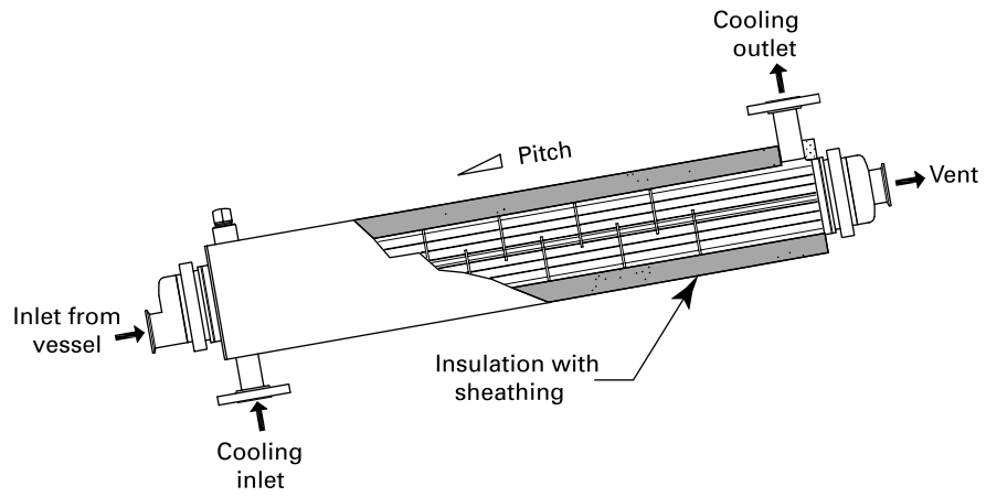
Figure SD-5.1.4.2.1-1 Exhaust Gas Condenser
