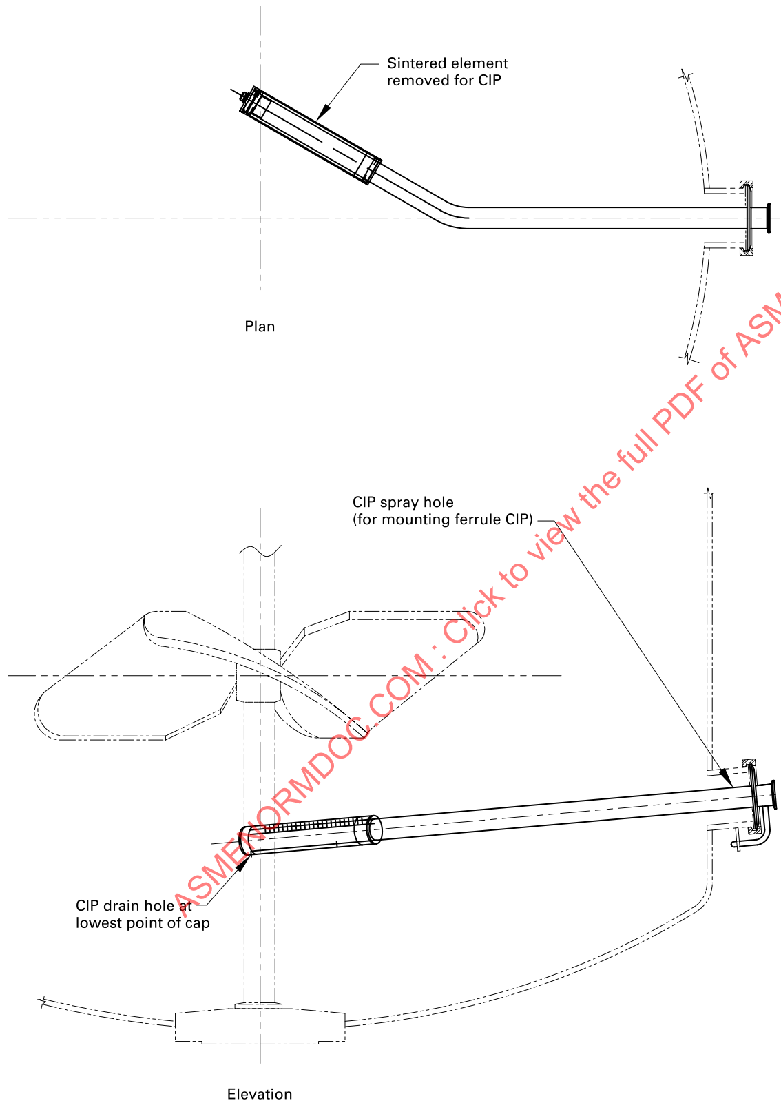
Figure SD-5.1.4.1.3-2 Gas Sparging Assembly — Sintered
