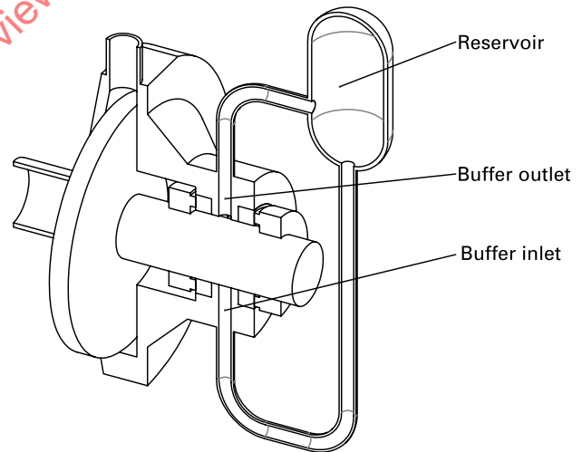
Figure MC-2.3.2.4-6 Plan 52 for Pump
