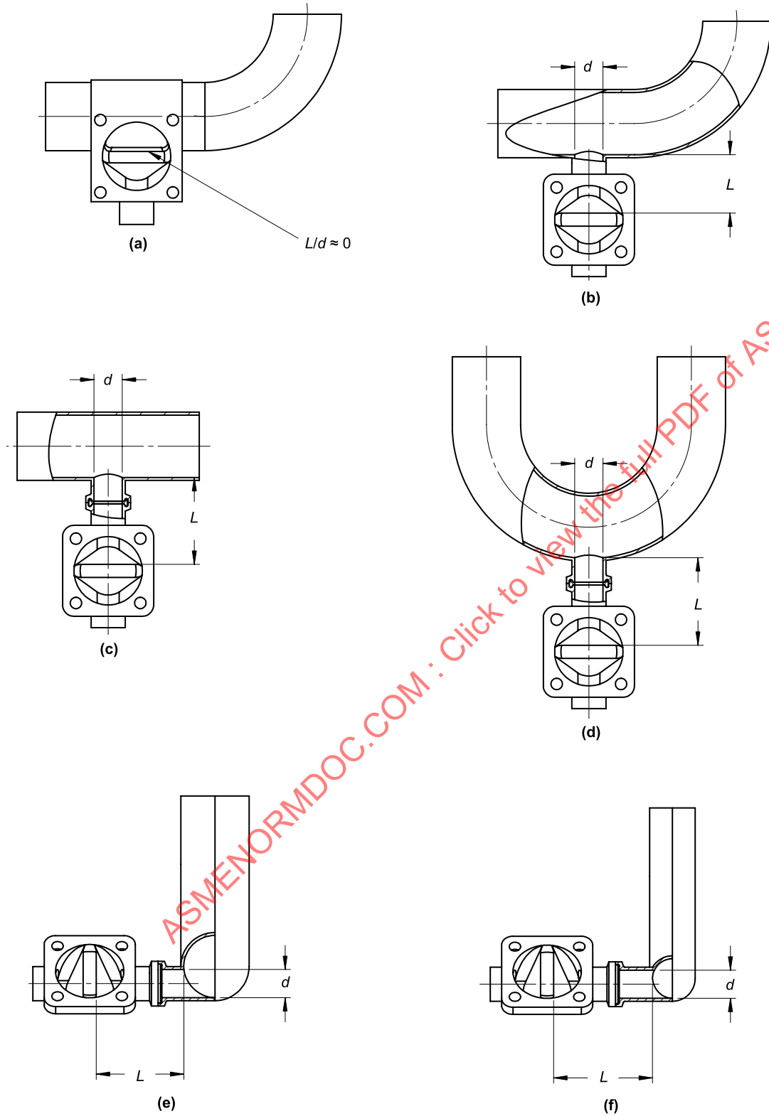
Figure SD-3.1.2.2-1 Accepted Point-of-Use Designs
