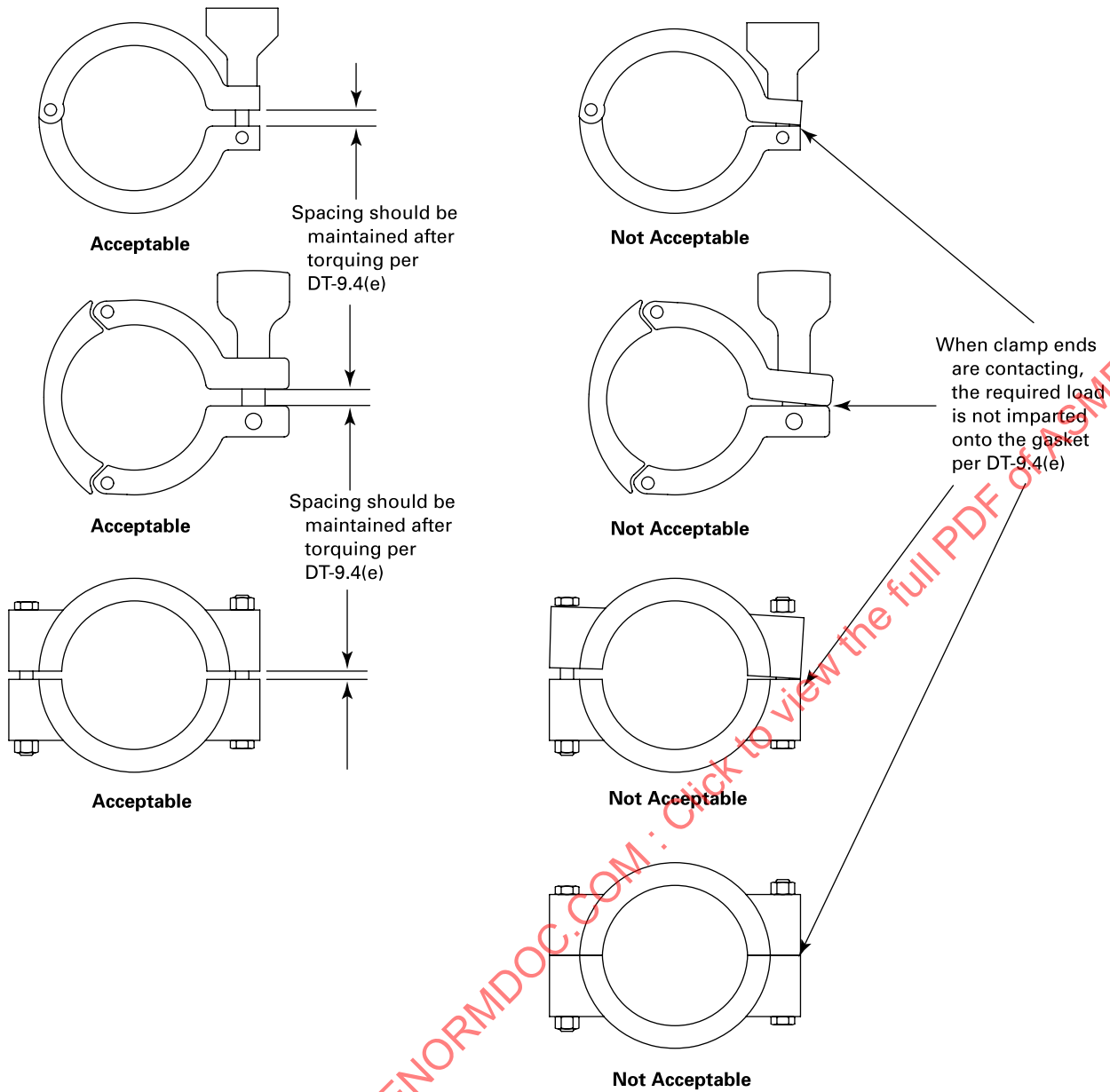
Figure DT-9.4-1 Clamp Conditions at Installation
