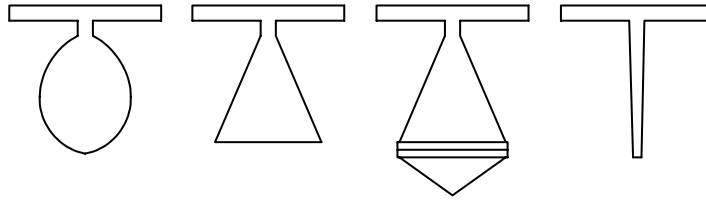
Figure PI-5.1.2-1 Bulb, Horn, Isolated Horn, and Rod-Style Antenna
