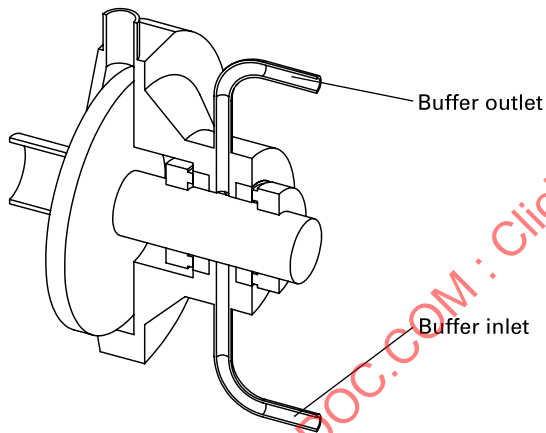
Figure MC-2.3.2.4-12 Plan 55 for Pump
