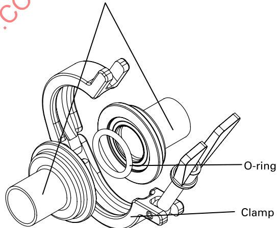
Figure MC-2.2.2-4 Hygienic Clamp Union per DIN 11864
