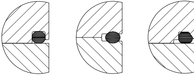
Figure MC-3.3.2.2-1 Examples of Static O-Ring Grooves
