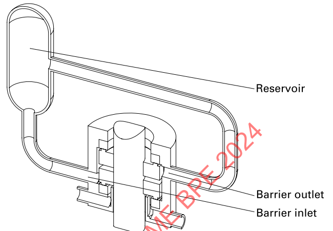
Figure MC-2.3.2.4-9 Plan 53 for Top-Entry Agitator
