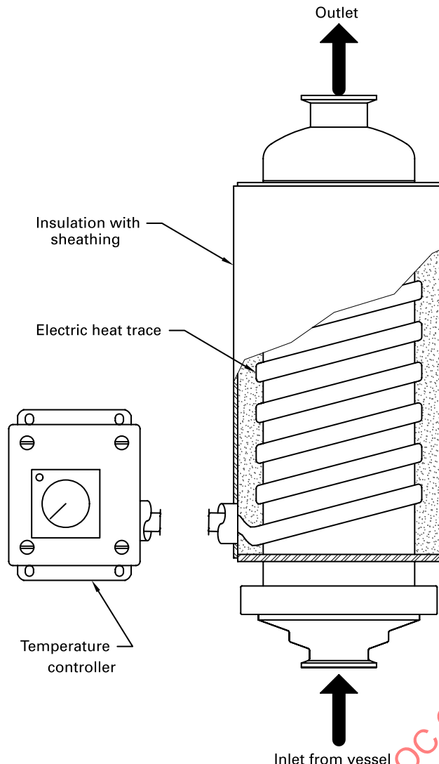
Figure SD-5.1.4.2.1-3 Electrically Heat Traced Filter Housing
