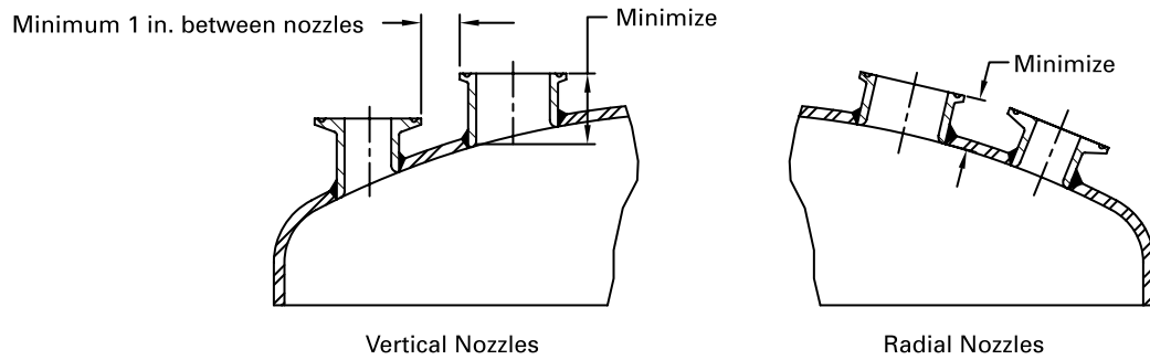
Figure SD-3.4.2-1 Nozzle Design
