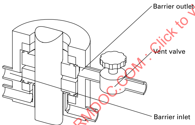
Figure MC-2.3.2.4-16 Plan 74 for Top-Entry Agitator
