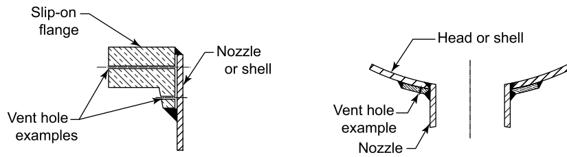
Figure MJ-3.1-1 Vent Hole Examples
