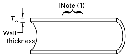
(a) Acceptable Weld Profile
