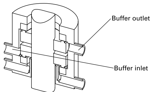
Figure MC-2.3.2.4-14 Plan 55 for Top-Entry Agitator
