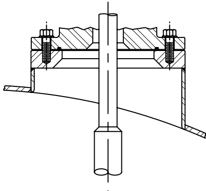
(a) Bolted Flange With O-Ring
