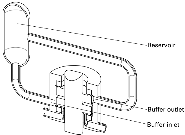
Figure MC-2.3.2.4-7 Plan 52 for Top-Entry Agitator
