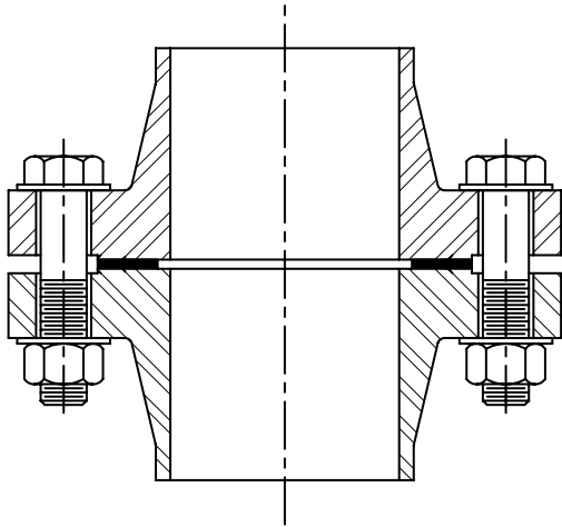
(a) Flange With Flat Gasket
