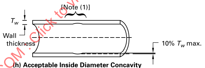
(h) Acceptable Inside Diameter Concavity
