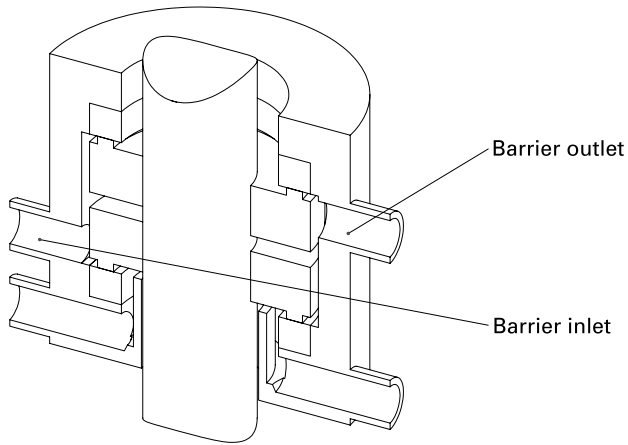
Figure MC-2.3.2.4-11 Plan 54 for Top-Entry Agitator
