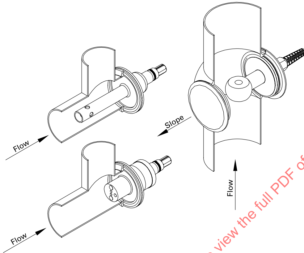
Figure PI-8.1.3.2-1 Acceptable Orientations for Conductivity Sensors
