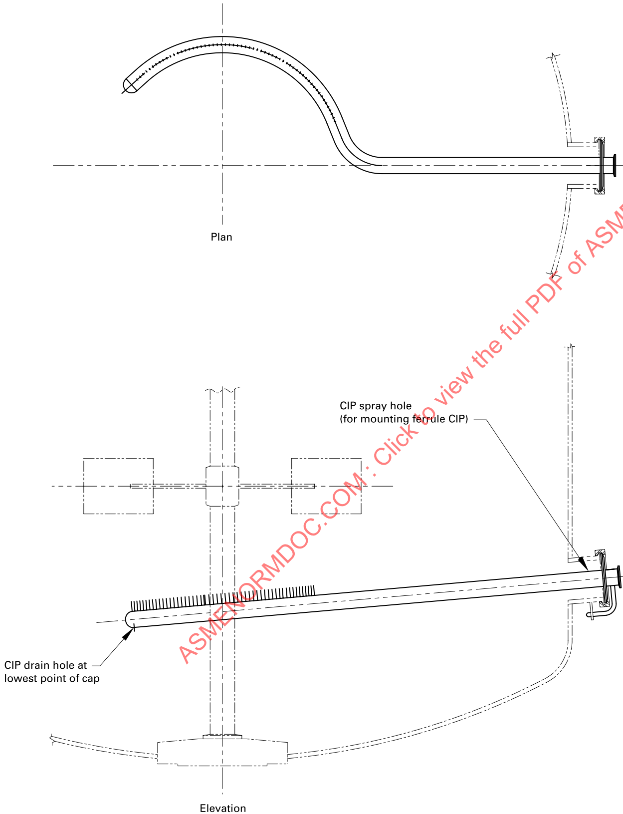
Figure SD-5.1.4.1.3-3 Gas Sparging Assembly — Ring
