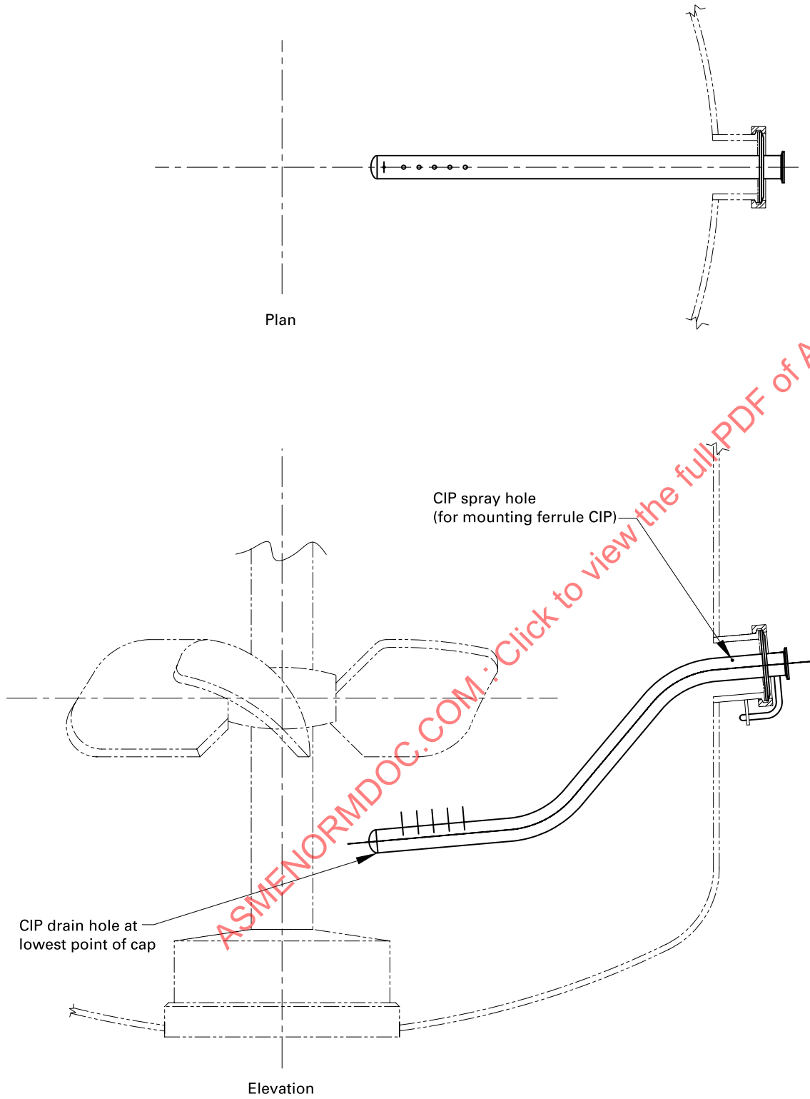
Figure SD-5.1.4.1.3-1 Gas Sparging Assembly — Lance
