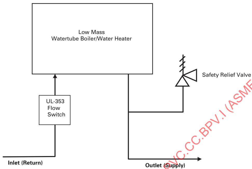
Figure 1 Alternate Safety Relief Valve Mounting
