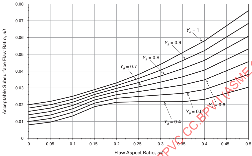
Figure 2 Alternative Subsurface Flaw Acceptance Criteria
