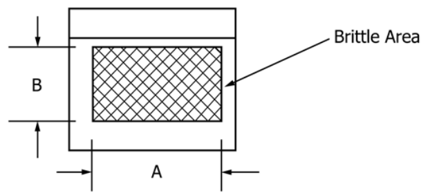
Measure Dimensions A and B to the nearest ½ mm. FIG. S5.1 Calculation of Percent Fibrous Area
