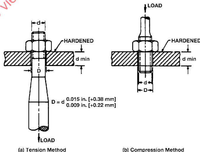
FIG. 1 Proof Load Testing—Nuts
