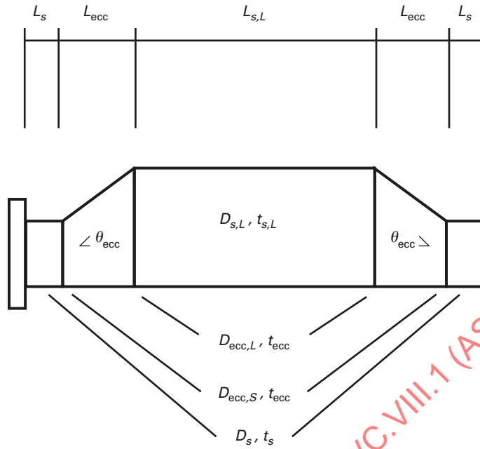
Figure UHX-13.10.3-1 Kettle Shell
