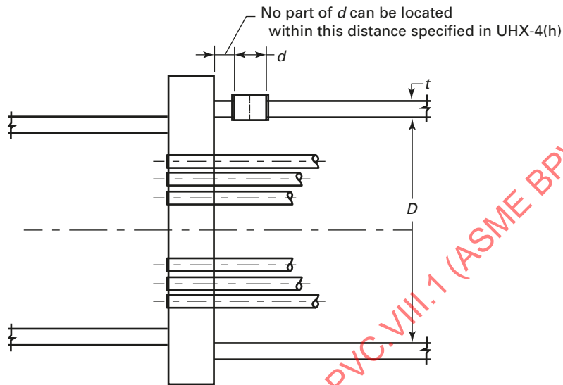
Figure UHX-4-1 Nozzles Adjacent to Tubesheets
