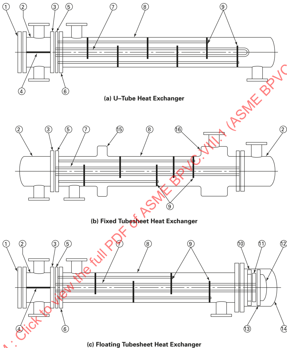
Figure UHX-3 Terminology of Heat Exchanger Components
