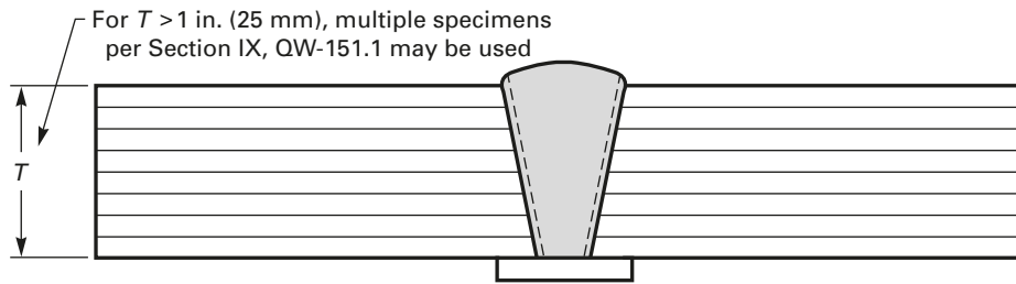
Figure ULW-32.2
