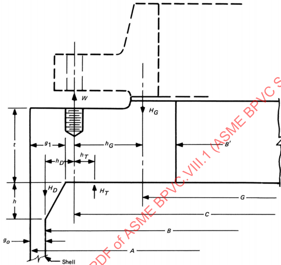
Figure 2-13.1 Reverse Flange
