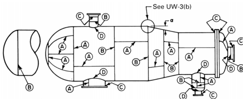
Figure UW-3
