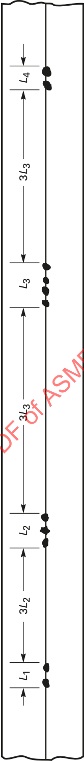
Figure 4-2 Groups of Aligned Rounded Indications
