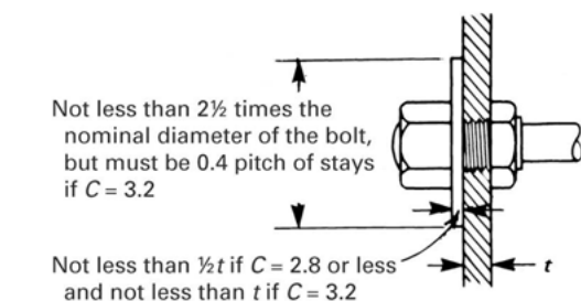
Figure UG-47 Acceptable Proportions for Ends of Stays
