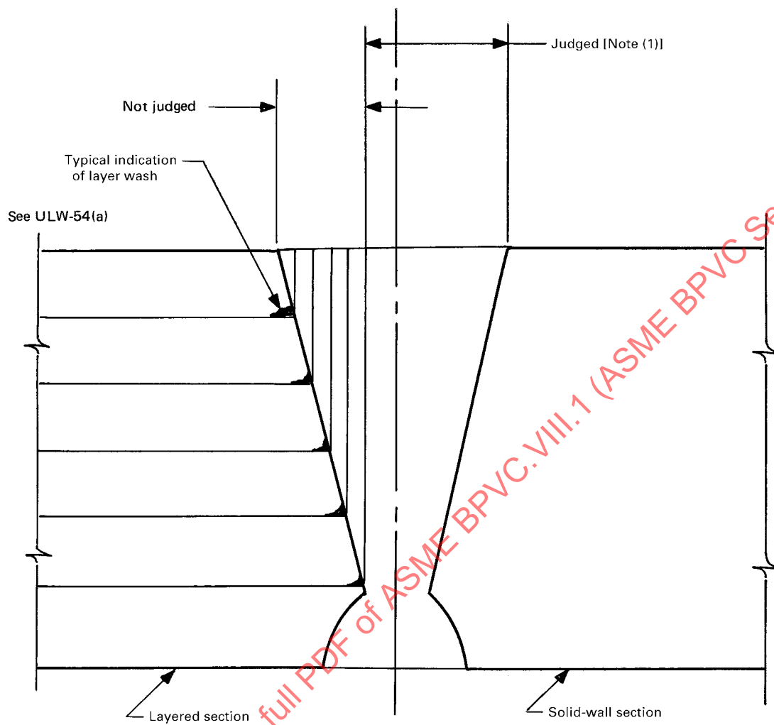
Figure ULW-54.1
