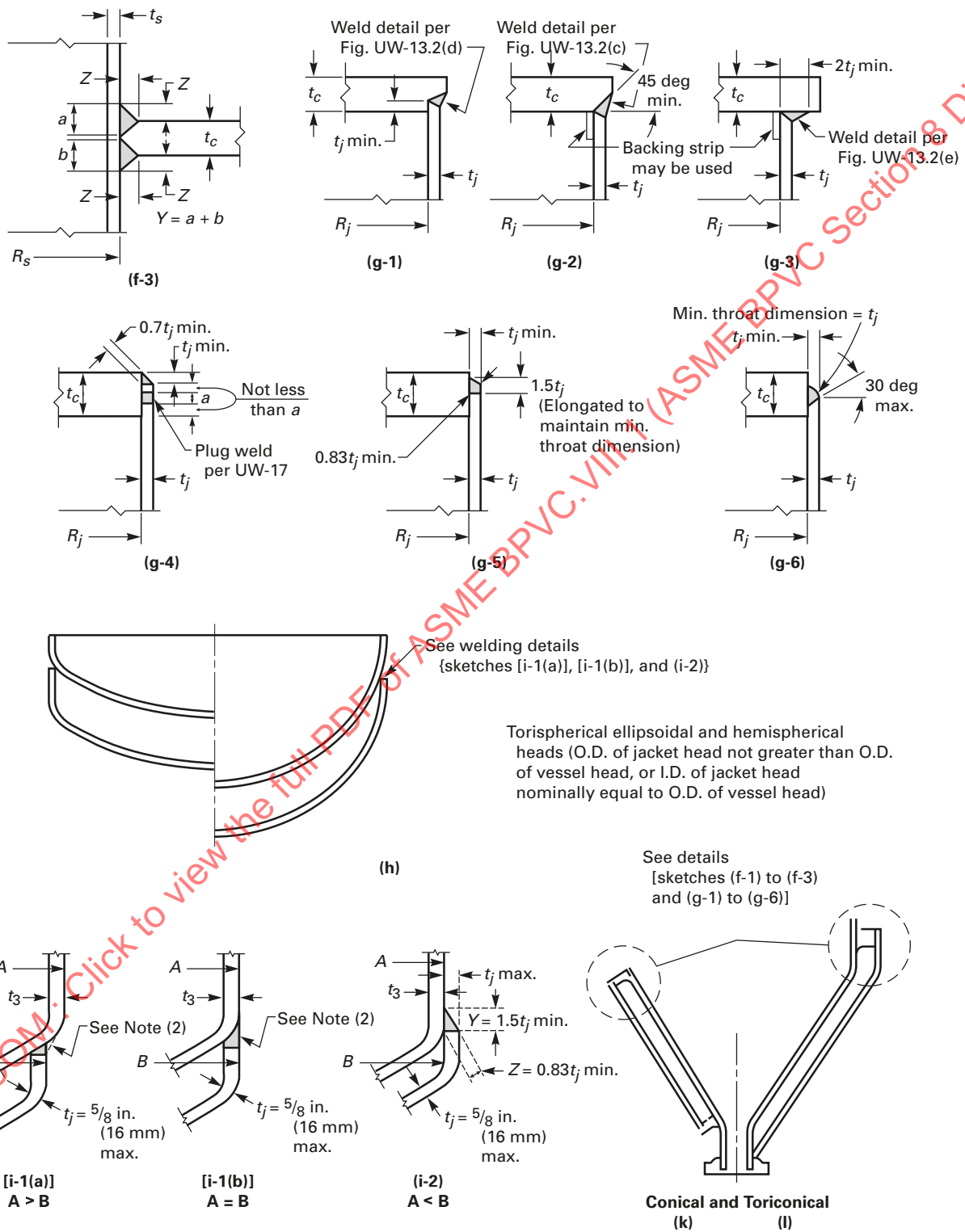
Figure 9-5 Some Acceptable Types of Jacket Closures (Cont'd)
