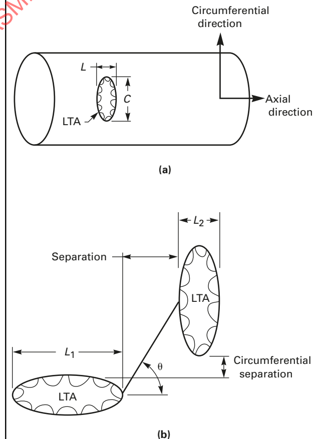
Figure 32-3 Nomenclature
