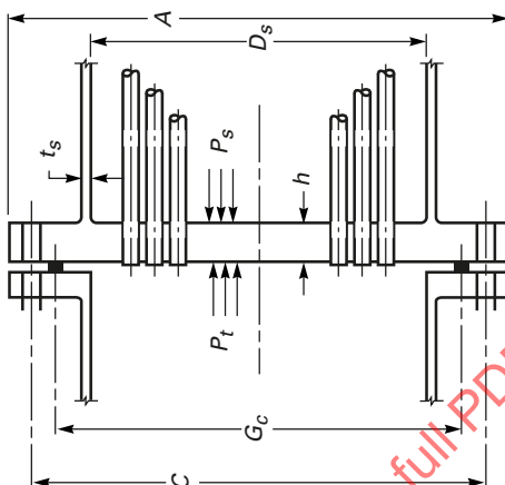
Figure UHX-12.1 U-Tube Tubesheet Configurations
