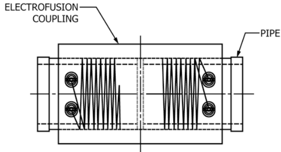
FIG. 2 Correct Wire Termination Coupling—Dual Coil
