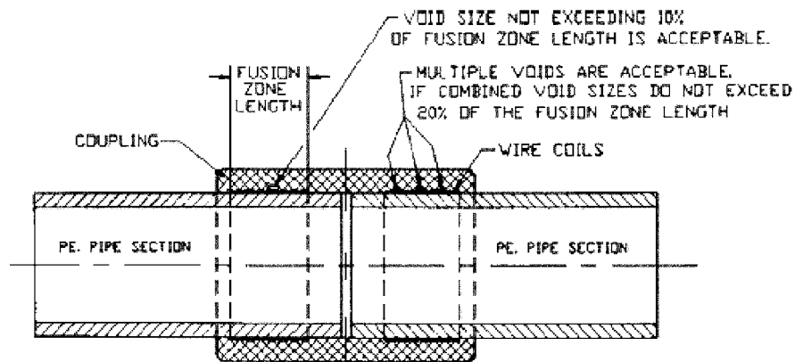
FIG. 10 Coupling Fusion Assembly With Possible Void Characteristics
