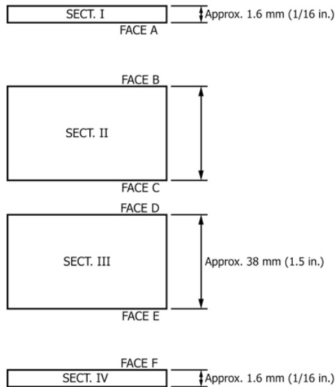
FIG. 4 Sectioned PTFE Test Billet
