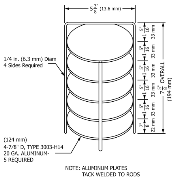
FIG. 2 SSG Samples Sintering Rack
