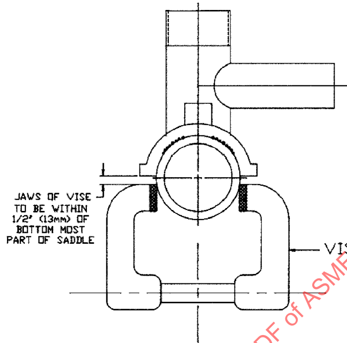
FIG. 5 Saddle Fitting Crush Test Before Crush
