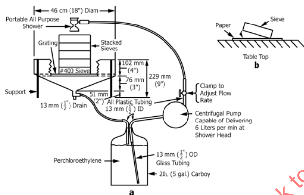
FIG. 9 Apparatus for Particle Size Test
