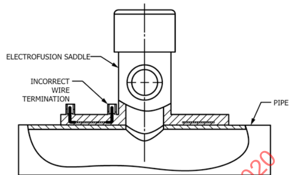
FIG. 5 Incorrect Wire Termination Saddle—Single Coil
