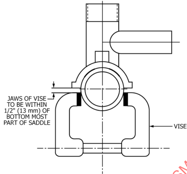
FIG. 5 Saddle Fitting Crush Test Before Crush
