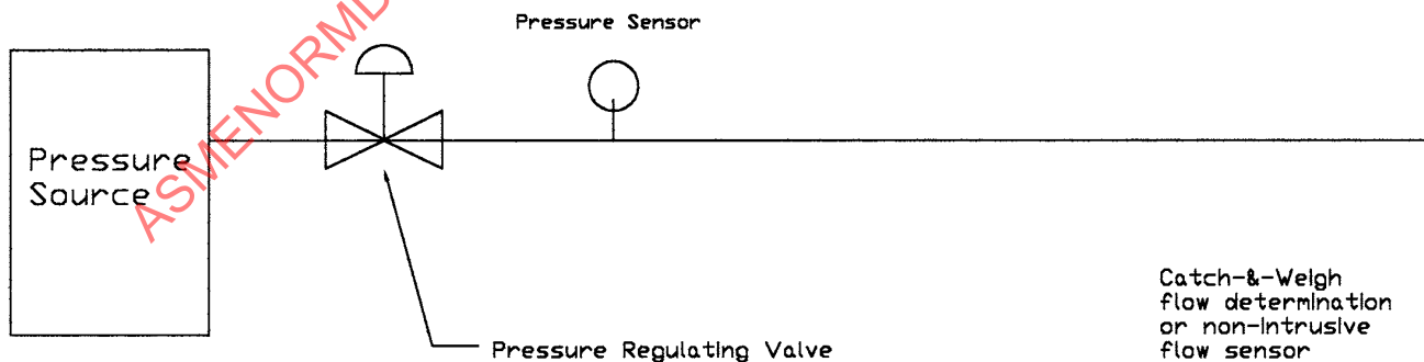
FIG. 3 Flow Without Test Valve
