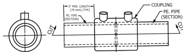
FIG. 6 Preparation of Coupling Specimen for Crush Test
