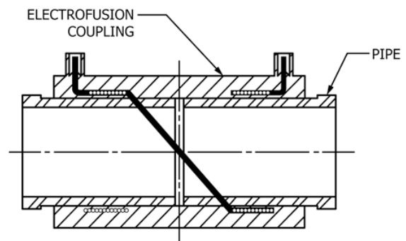
FIG. 1 Correct Wire Termination Coupling—Single Coil
