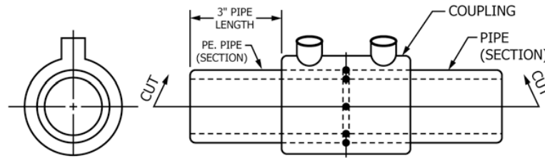
FIG. 1 Preparation of Coupling Specimen for Crush Test
