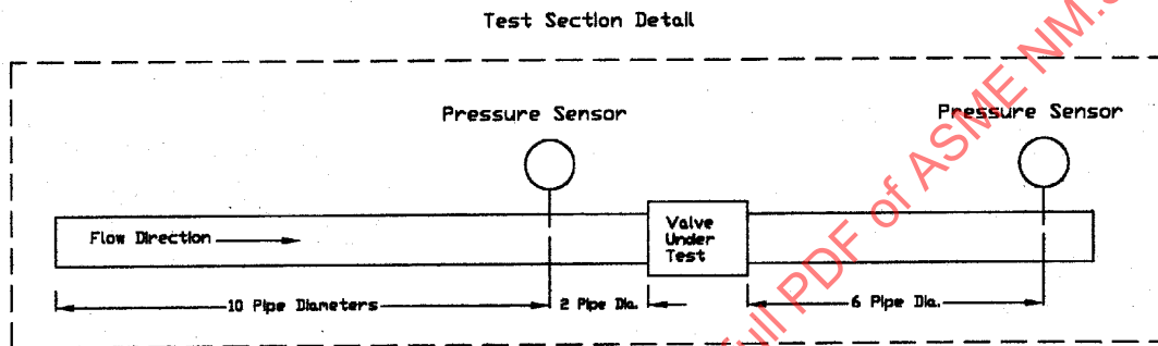
FIG. 1 Pressure Loss Test System
