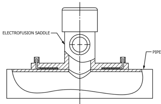
FIG. 3 Correct Wire Termination—Saddle Fitting
