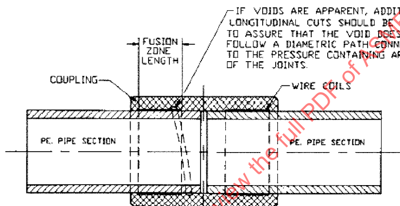
FIG. 11 Coupling Fusion Assembly—Further Examination Guidance
