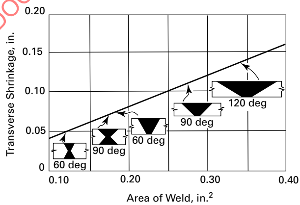
Fig. 2 Effect of Weld Area on Transverse Shrinkage
