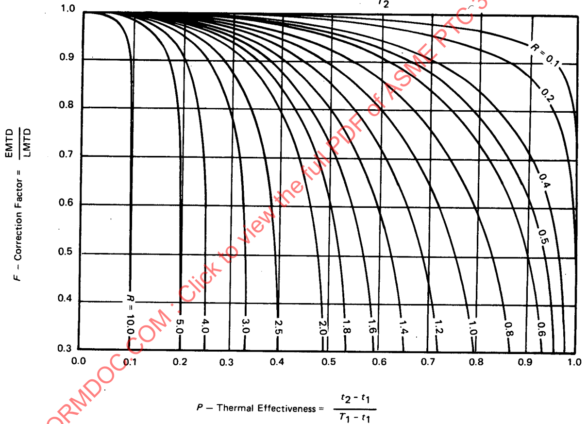
FIG. 5.4 MEAN TEMPERATURE DIFFERENCE RELATIONSHIPS Crossflow Unit – 4 Tube Rows, 1 Pass, Unmixed (Reproduced by permission of Heat Transfer Research, Inc.)
