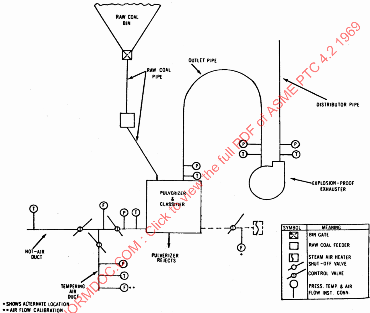
FIG. 2 EQUIPMENT ARRANGEMENT DIRECT-FIRED-SUCTION TYPE
