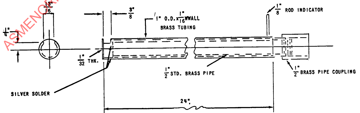
FIG. 5 DETAIL OF SAMPLING TIP
