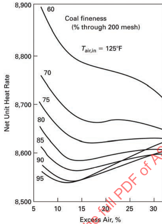
Fig. 1-2.6-10 Effect of O 2 and Coal Fineness on Unit Heat Rate (Courtesy Electric Power Research Institute)
