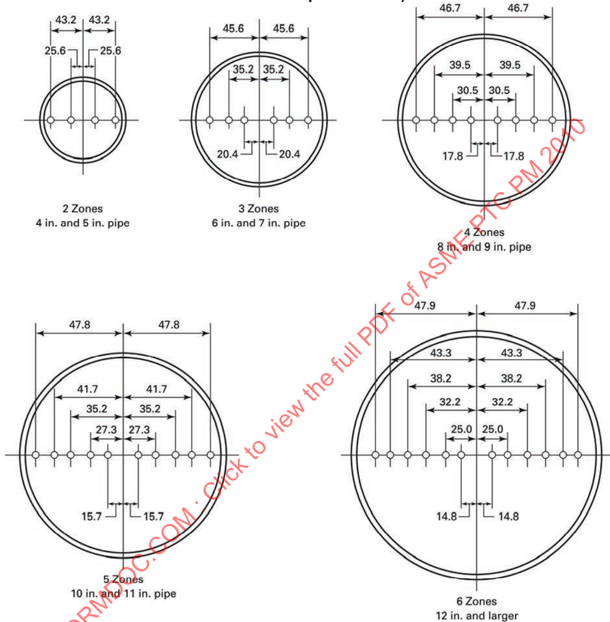
Fig. 2-3.8.6.1-1 Sampling Direct-Fired Pulverized Coal-Sampling Stations (Dimensions Are “Percent of Pipe Diameter”)
