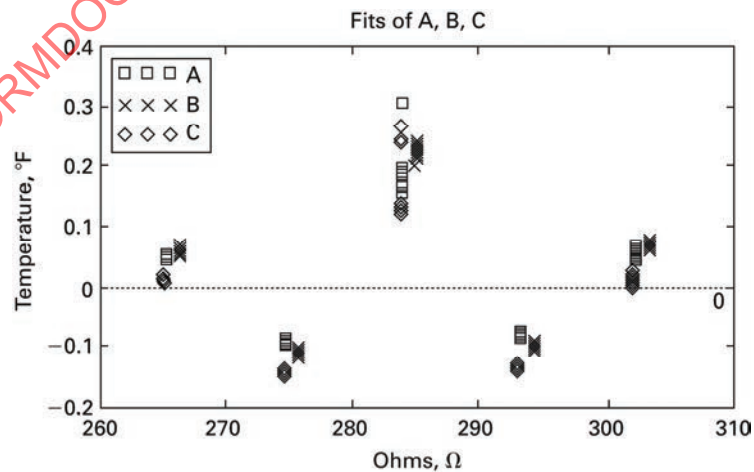
Fig. 3-3.2-4 Distribution of Errors for the Three RTDs
