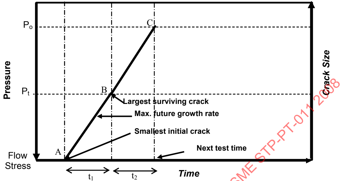
Figure 4 - Extrapolating the Maximum Prior Crack Growth Rate to Establish the Interval for the Next Re-Test
