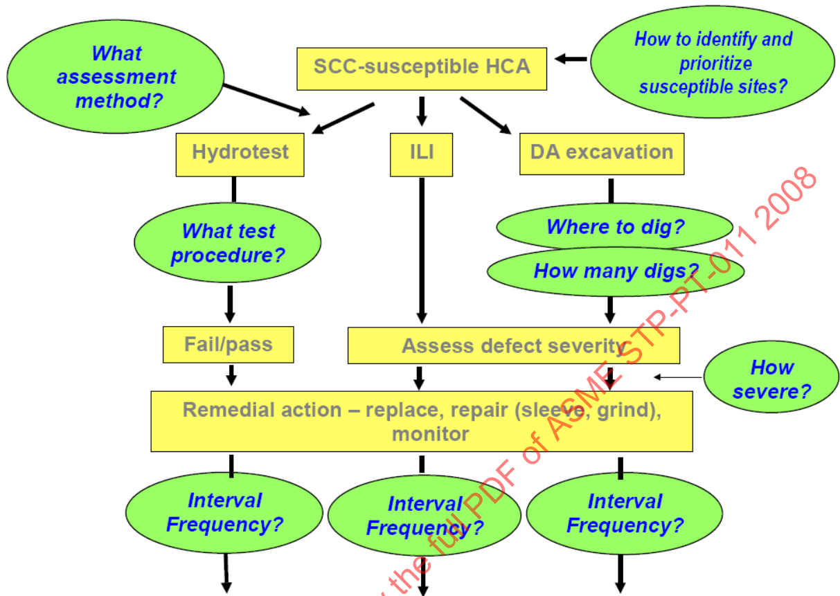
Figure 1 - Questions Arising During SCC Integrity Management
