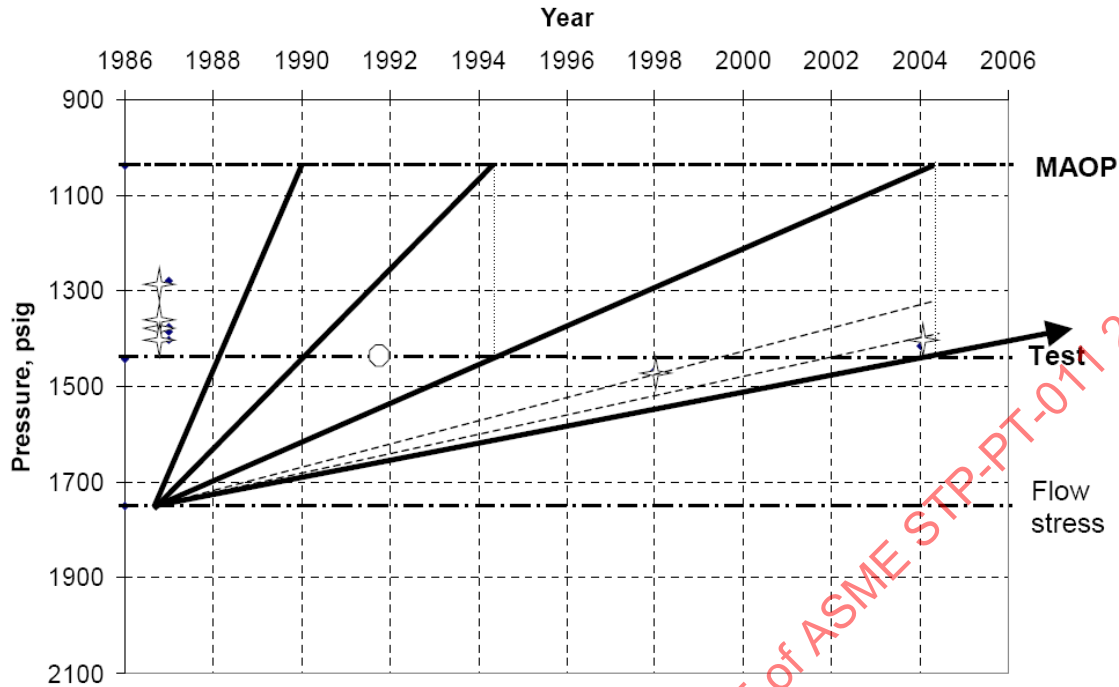
Figure 8 - Comparison of Service History with Predictions of this Method for Case 1 (Symbols are as described for Figure 7)
