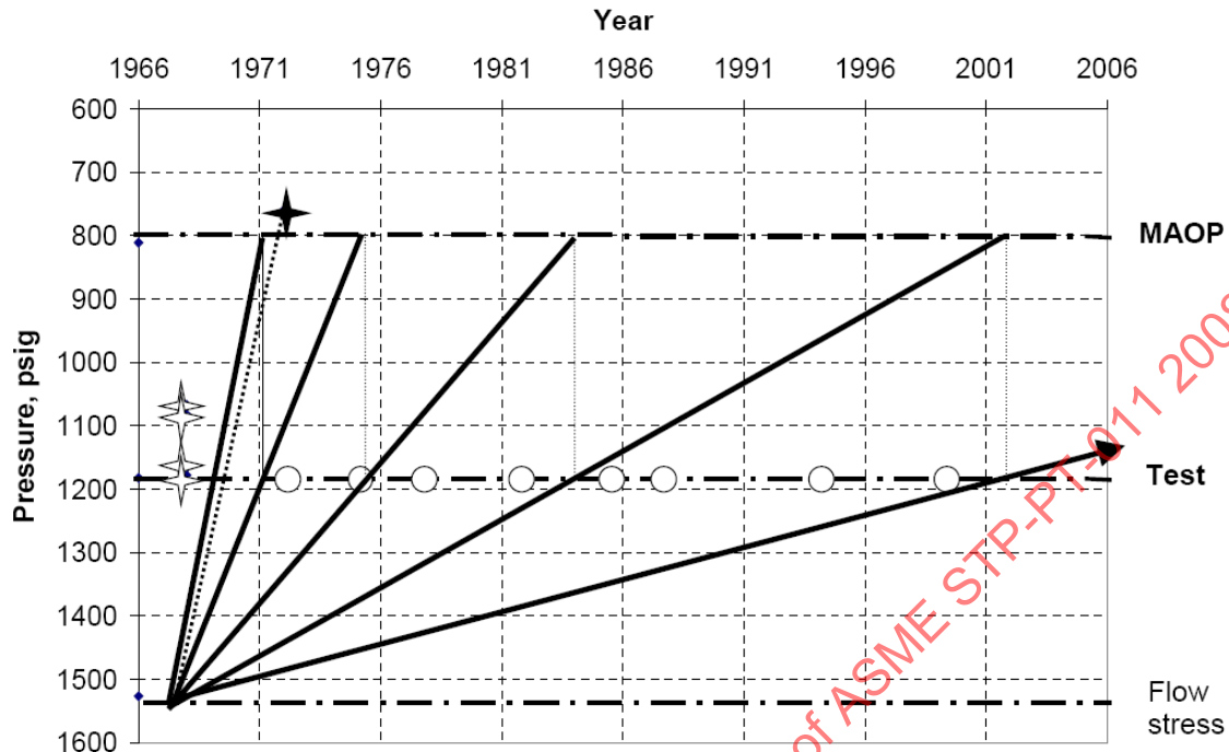
Figure 7 - Comparison of Service History with Predictions of this Method for Case 6
