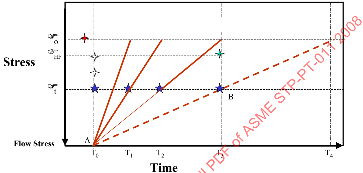
Figure 11 - Hypothetical Re-Test History to Illustrate Modification to Method Following a Re-Test Failure
