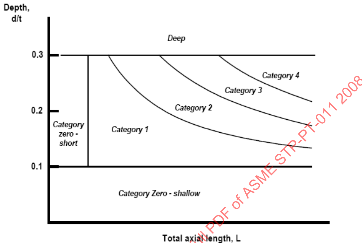
Figure 15 - Relation of Severity Categories to Crack Lengths and Depths (Schematic)
