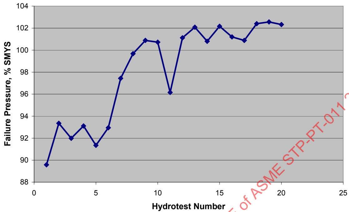
Figure 14 - Sequence of Failure Pressures in a Hydrostatic Test in which 20 Ruptures Initiated at Stress-Corrosion Cracks
