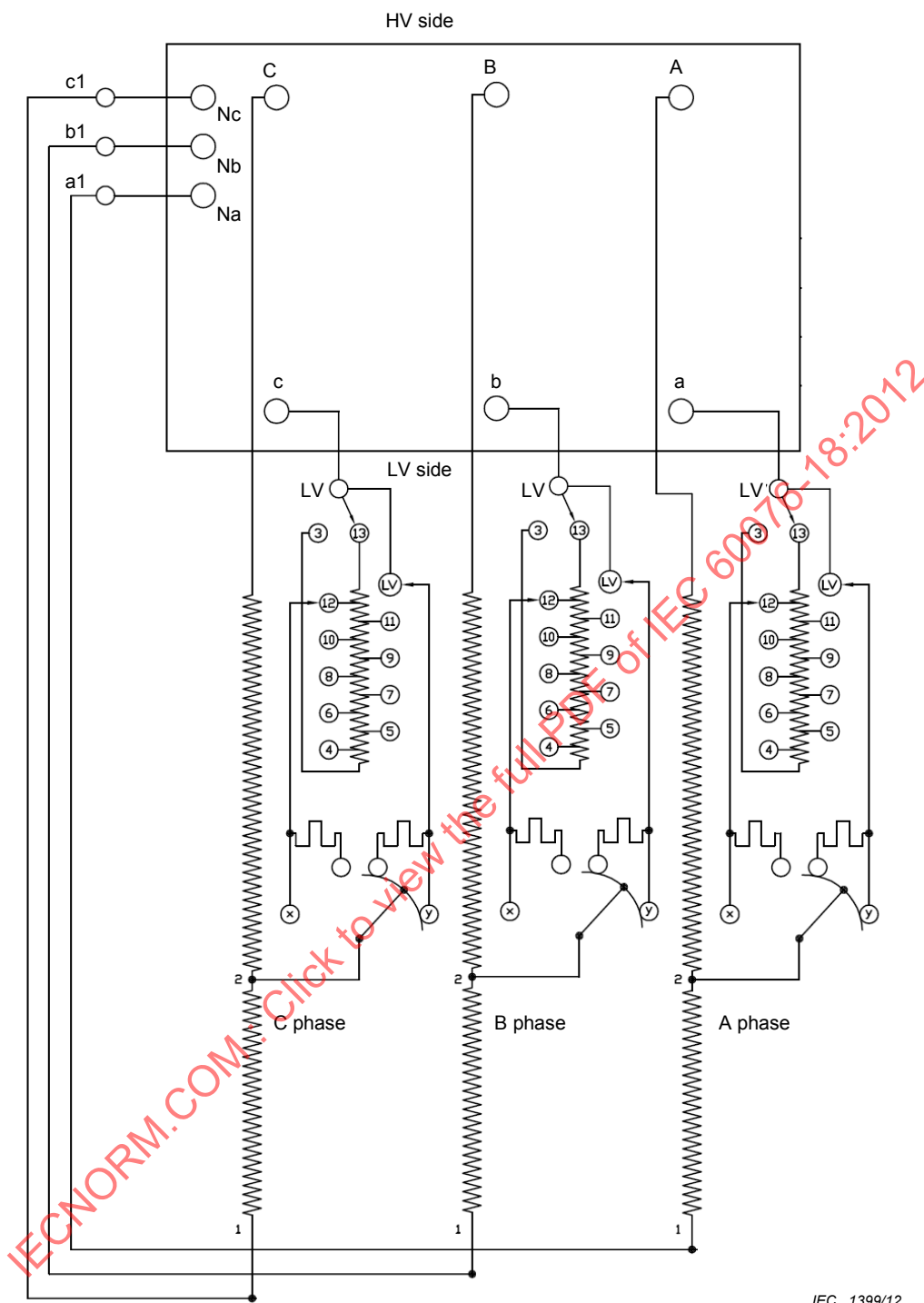
Figure D.1 – Winding diagram of an auto-transformer with a line-end tap changer
