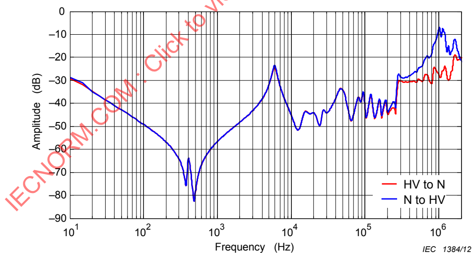
Figure B.11 – Effect of measurement direction on frequency response
