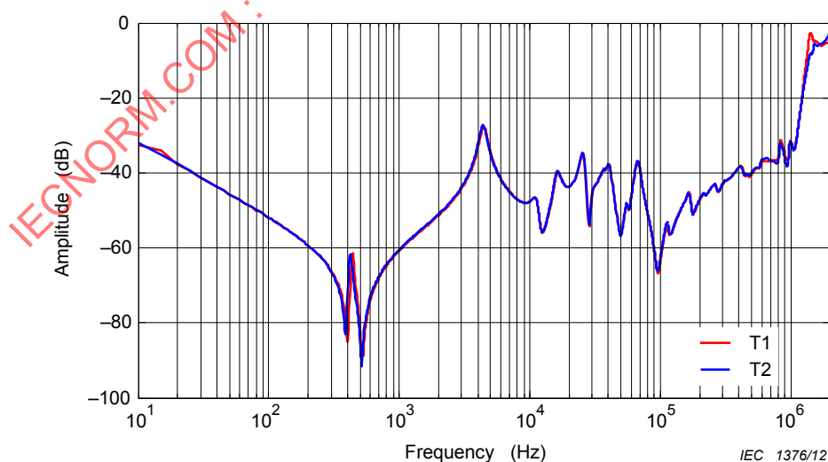
Figure B.3 – Comparison of the frequency responses of twin transformers
