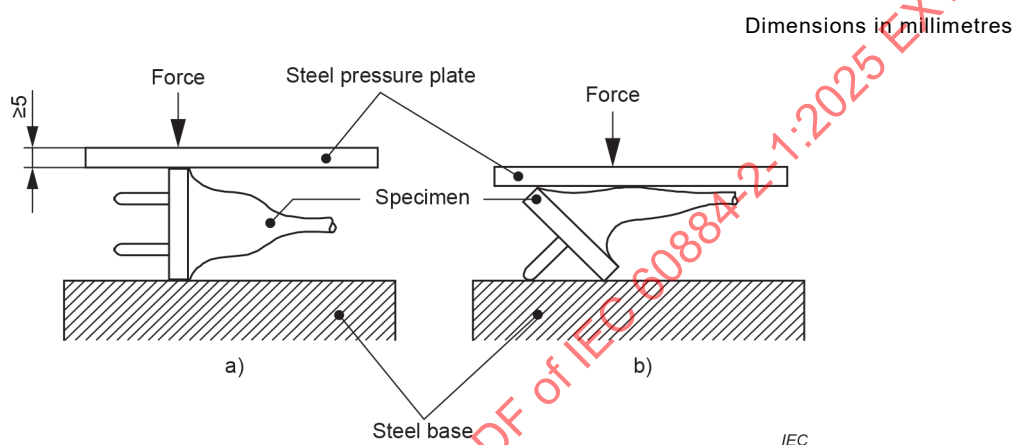
Figure 6 – Arrangement for compression test
