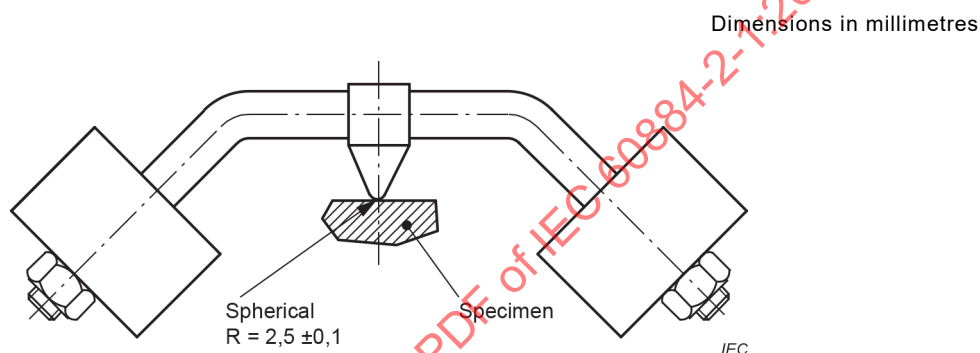
Figure 40 – Ball pressure test apparatus
