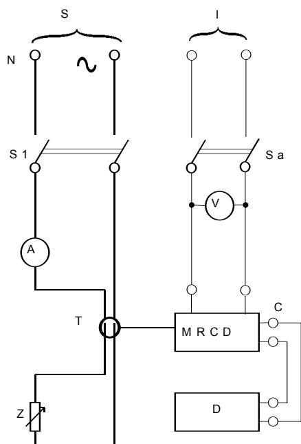
MRCD with separate sensing means
