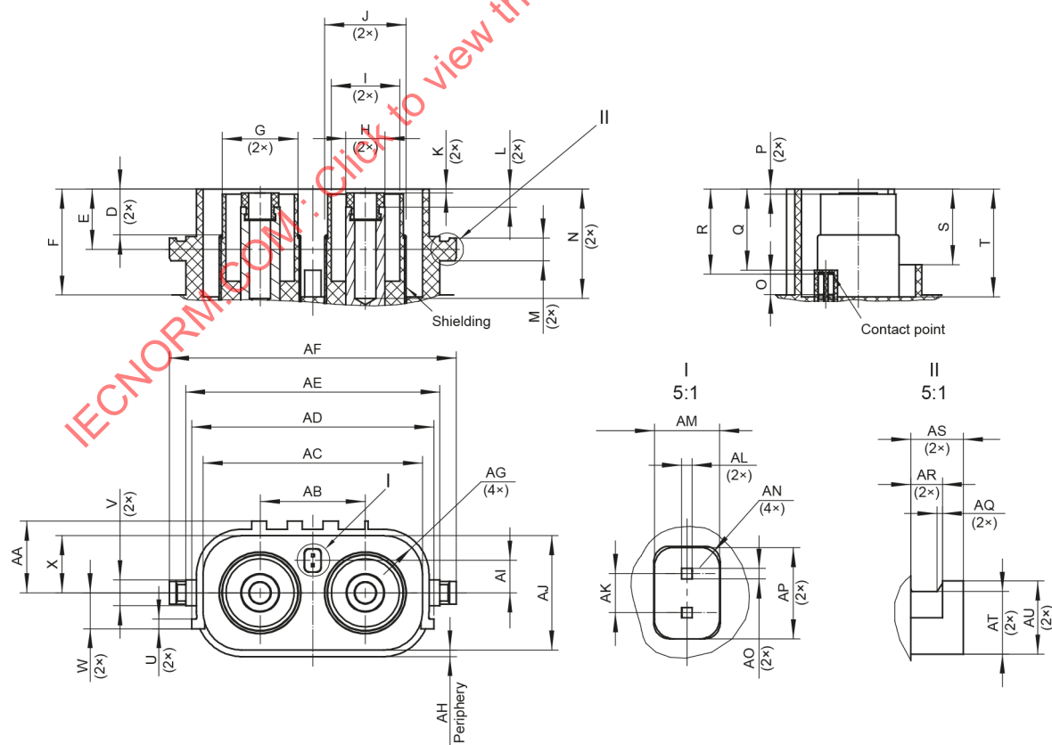
Figure 5 – Fixed connector
