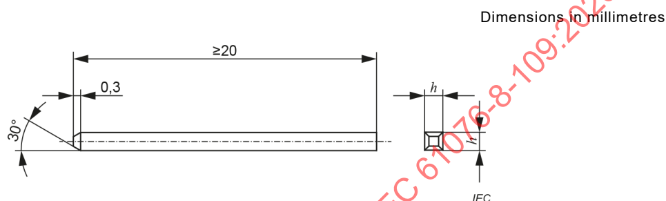
Figure 7 – Gauge for signal contacts
