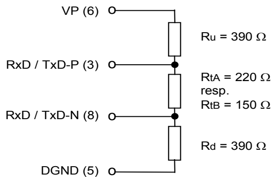
Figure 102 – Bus terminator
