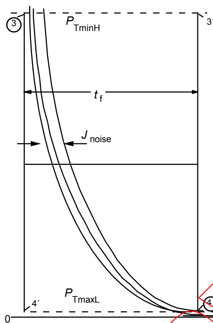
Figure 129 – Display of jitter ( J_{noise} )
