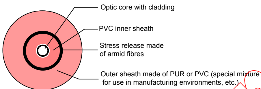
Figure O.2 – Structure of a single-core cable (example)
