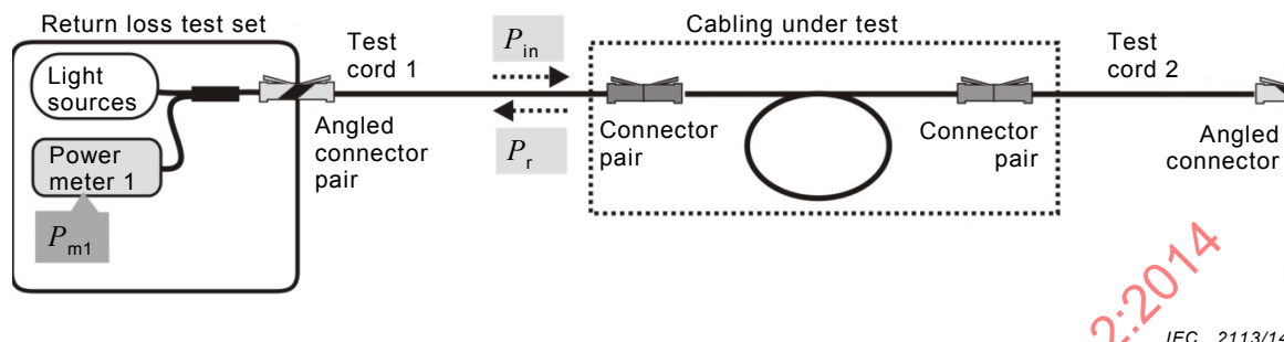
Figure F.5 – Measurement of the reflected power
