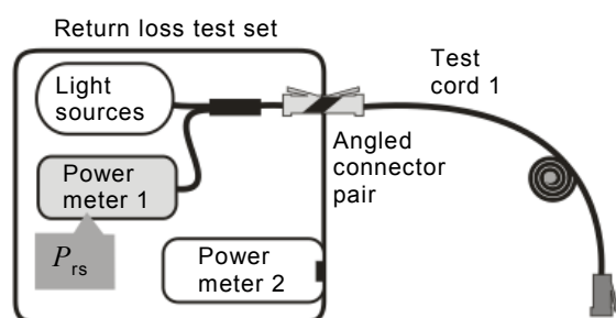
Figure E.4 – Measurement of the system reflected power P_{\text{rs}}
