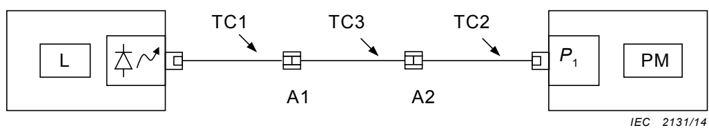
Figure I.11 – Obtaining power level P_1
