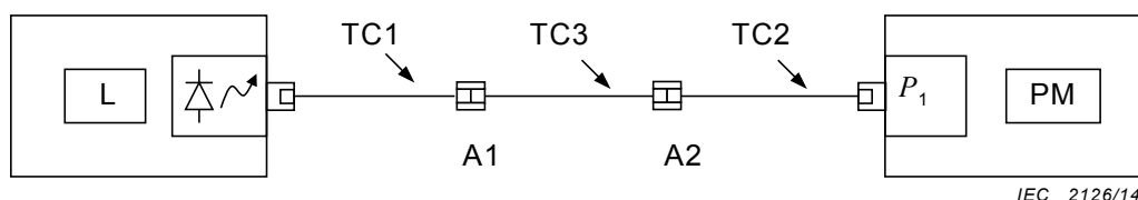
Figure I.6 – Obtaining power level
