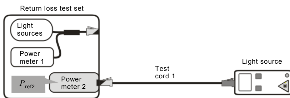
Figure E.2 – Measurement of the system internal attenuation P_{\text{ref2}}
