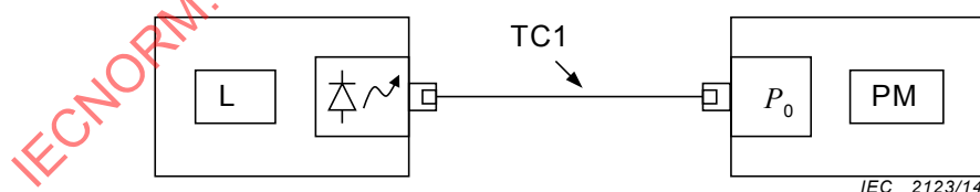
Figure I.3 – Obtaining reference power level P_0
