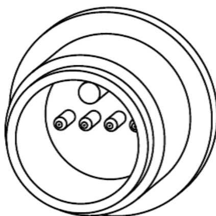
Figure 7 – Four way socket connector (isometric view)
