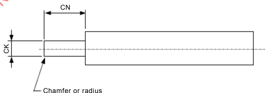
Figure 10 – Pin gauge for plug connector
