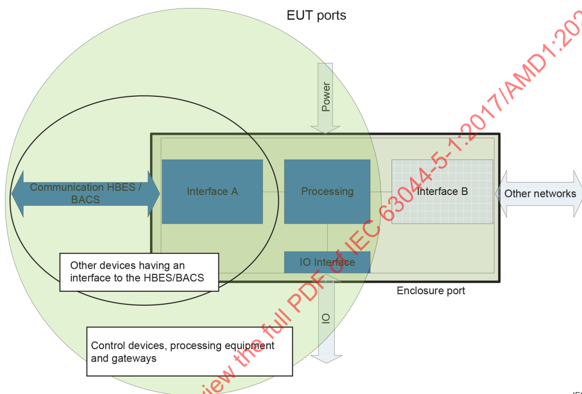
Figure 1 – EUT ports
