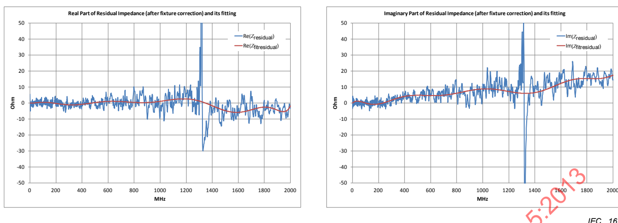
Figure 9 – Residual impedance (after fixture correction) and its fitting
