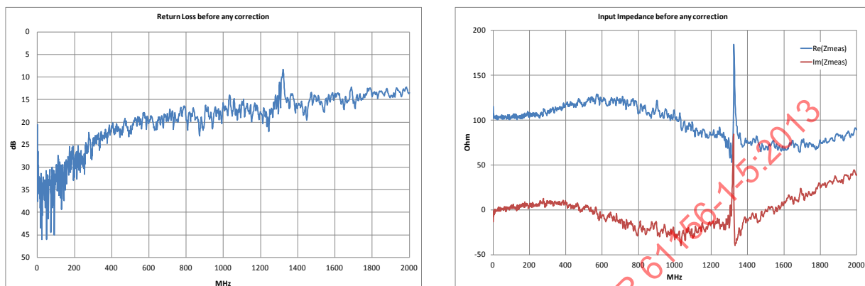
Figure 7 – Return loss and input impedance before any correction
