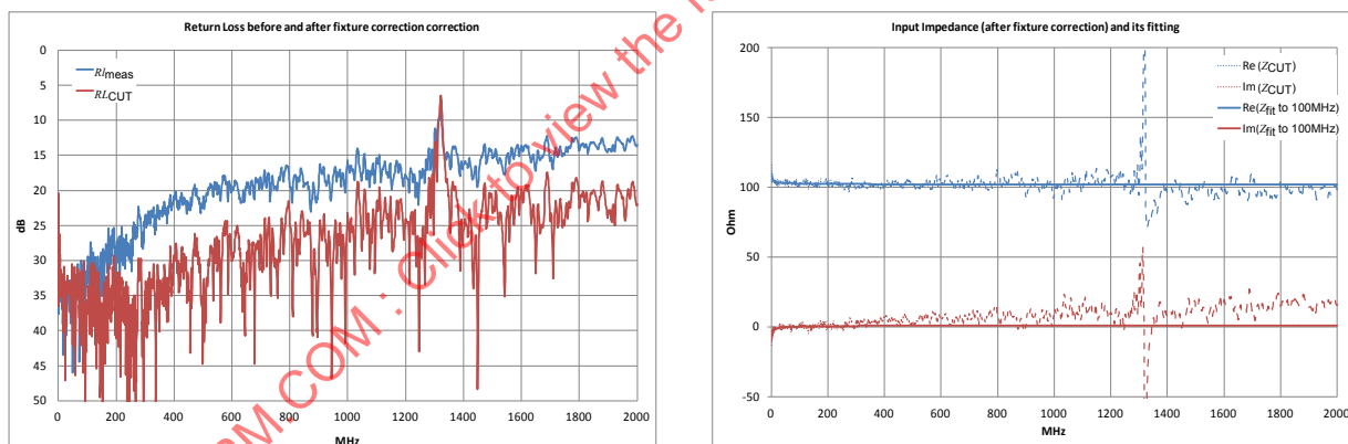
Figure 8 – Return loss and input impedance (with fitting) after fixture correction
