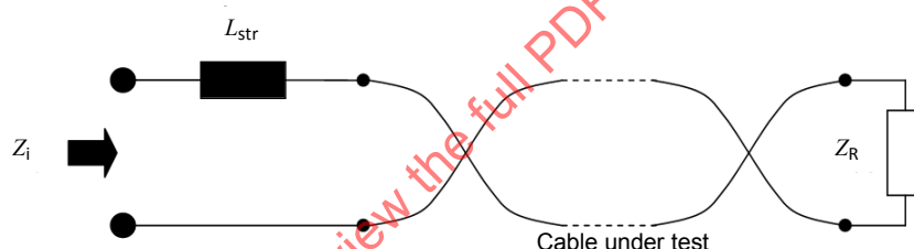
Figure 5 – Equivalent circuit for the corrective calculation
