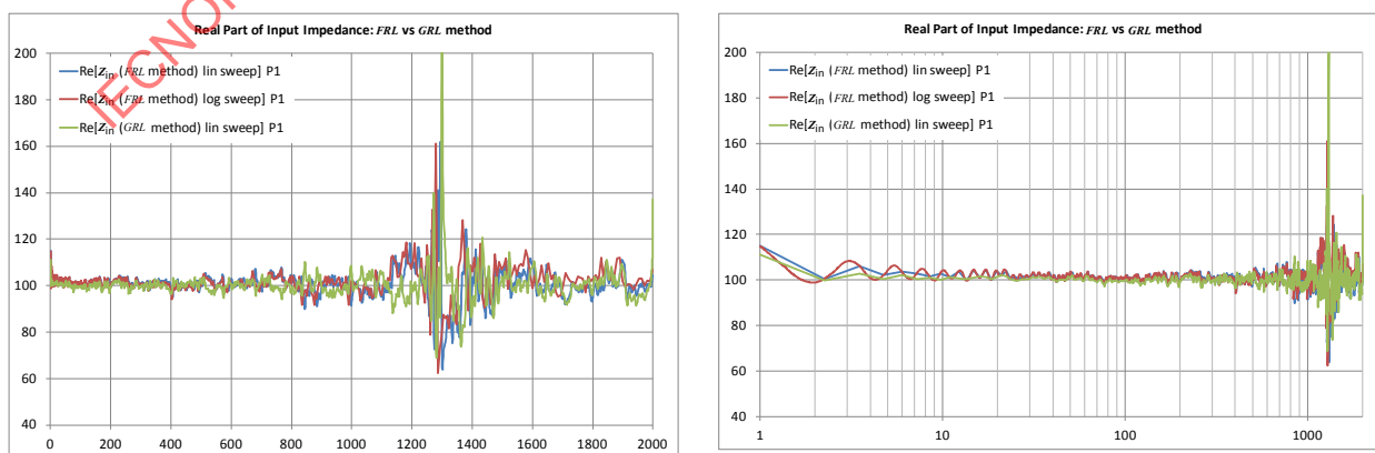
Figure A.2 – Real part of input impedance, fitting vs. gating correction
