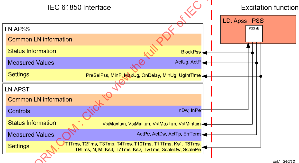
Figure 13 – Power system stabilizer function
