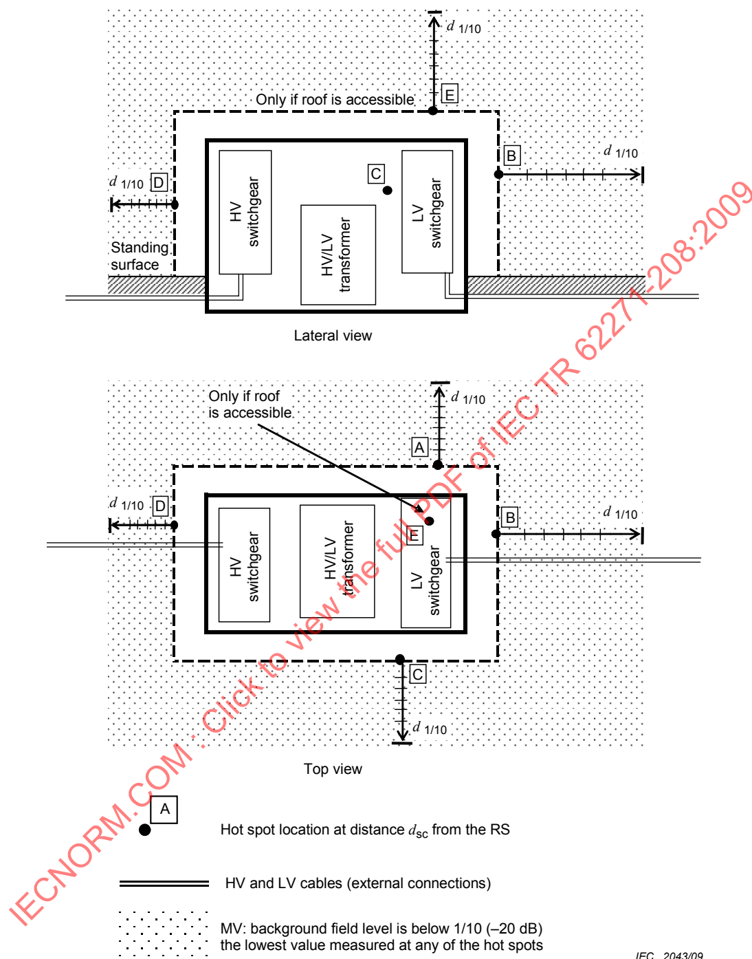
Figure 5 – Test set-up of main components, external cables, hot spot locations and measurement volume
