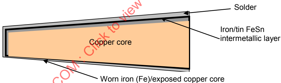
Figure 2 – Worn soldering iron tip
