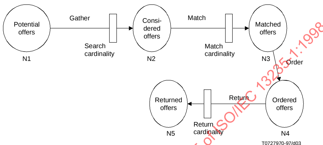
Figure 3 – Pipeline view of trader query steps and cardinality constraint application
