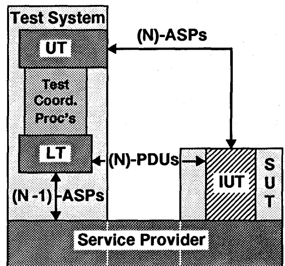
Figure 5 - The LS test method
