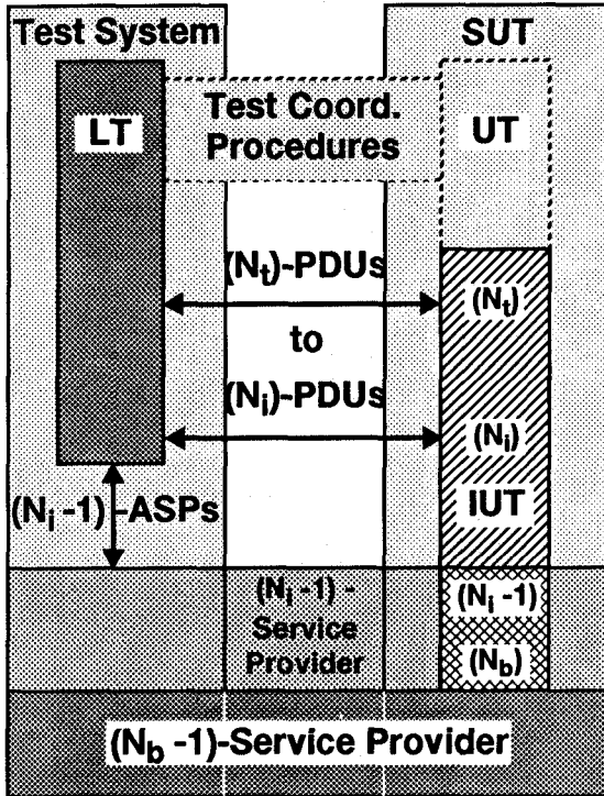
Figure 12 - Example of the RSE test method: testing the (N_i) -protocol in an (N_b) to (N_j) -protocol IUT
