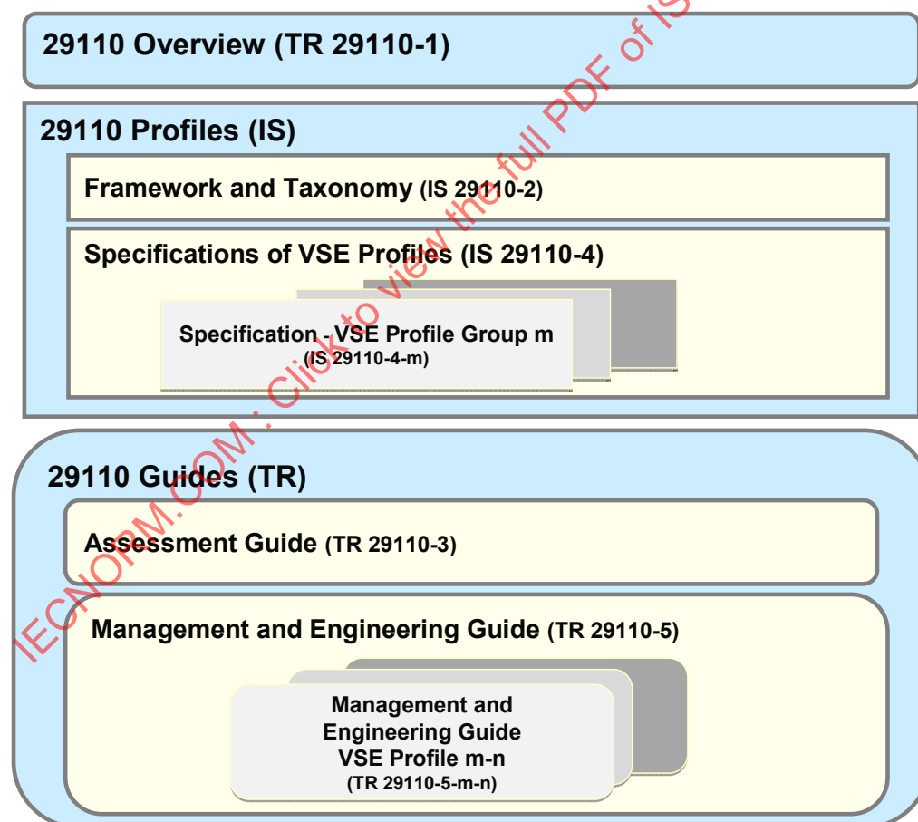
Figure 1 — ISO/IEC 29110 series
