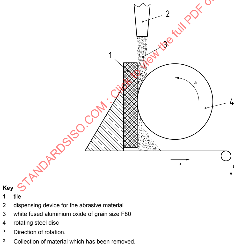
Figure 1 —Schematic diagram of deep abrasion equipment
