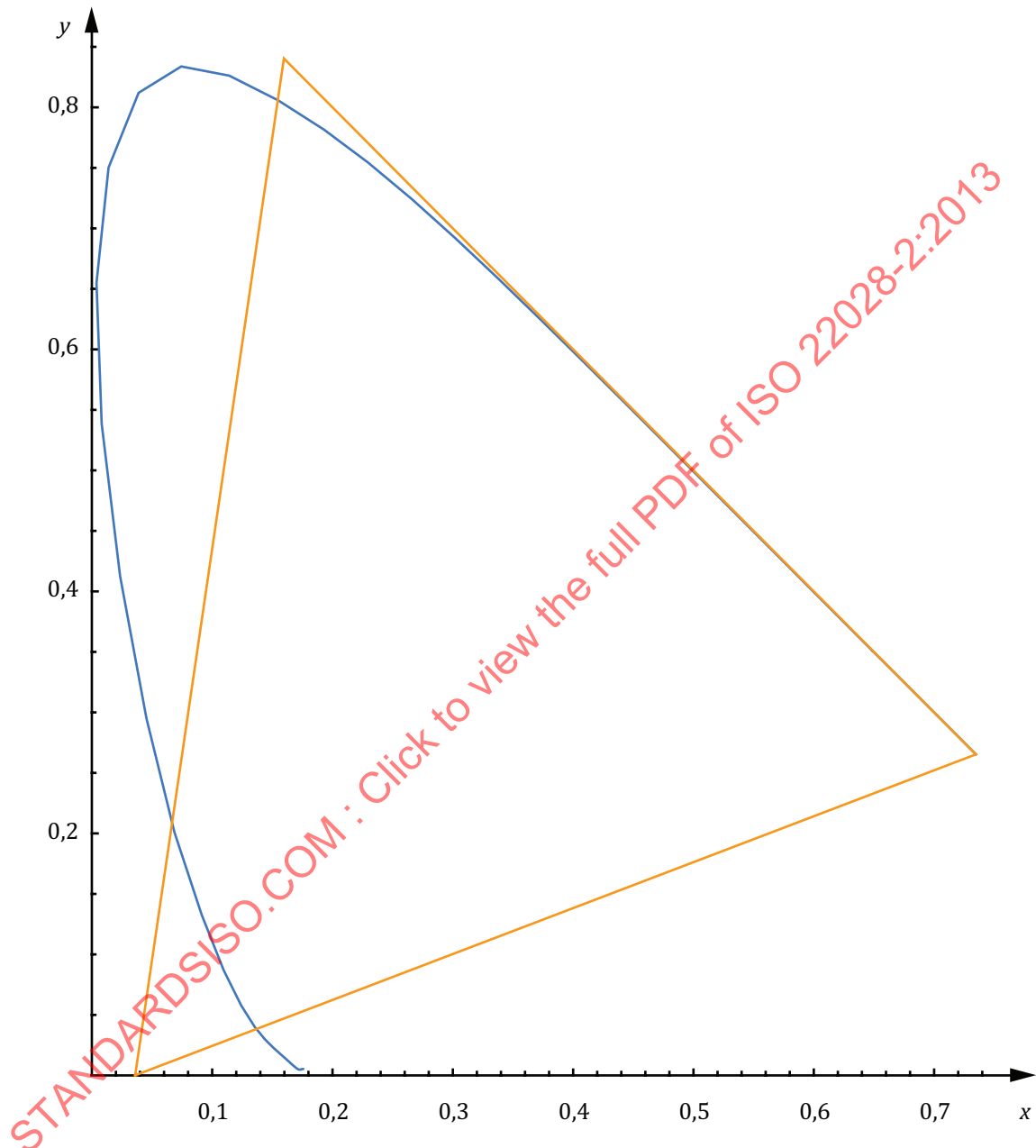
Figure 1 — x,y chromaticity plot of the spectrum locus and the ROMM RGB encoding gamut
