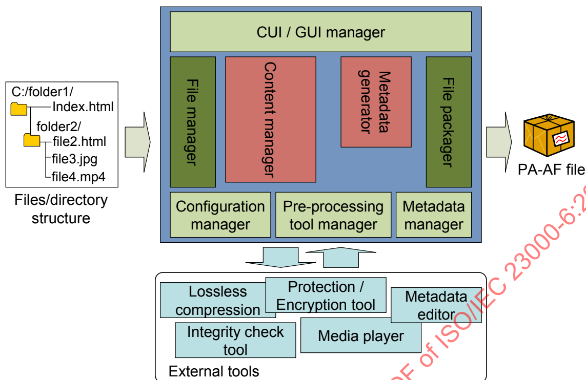
Figure 9 — A PA-AF packager/authoring tool architecture
