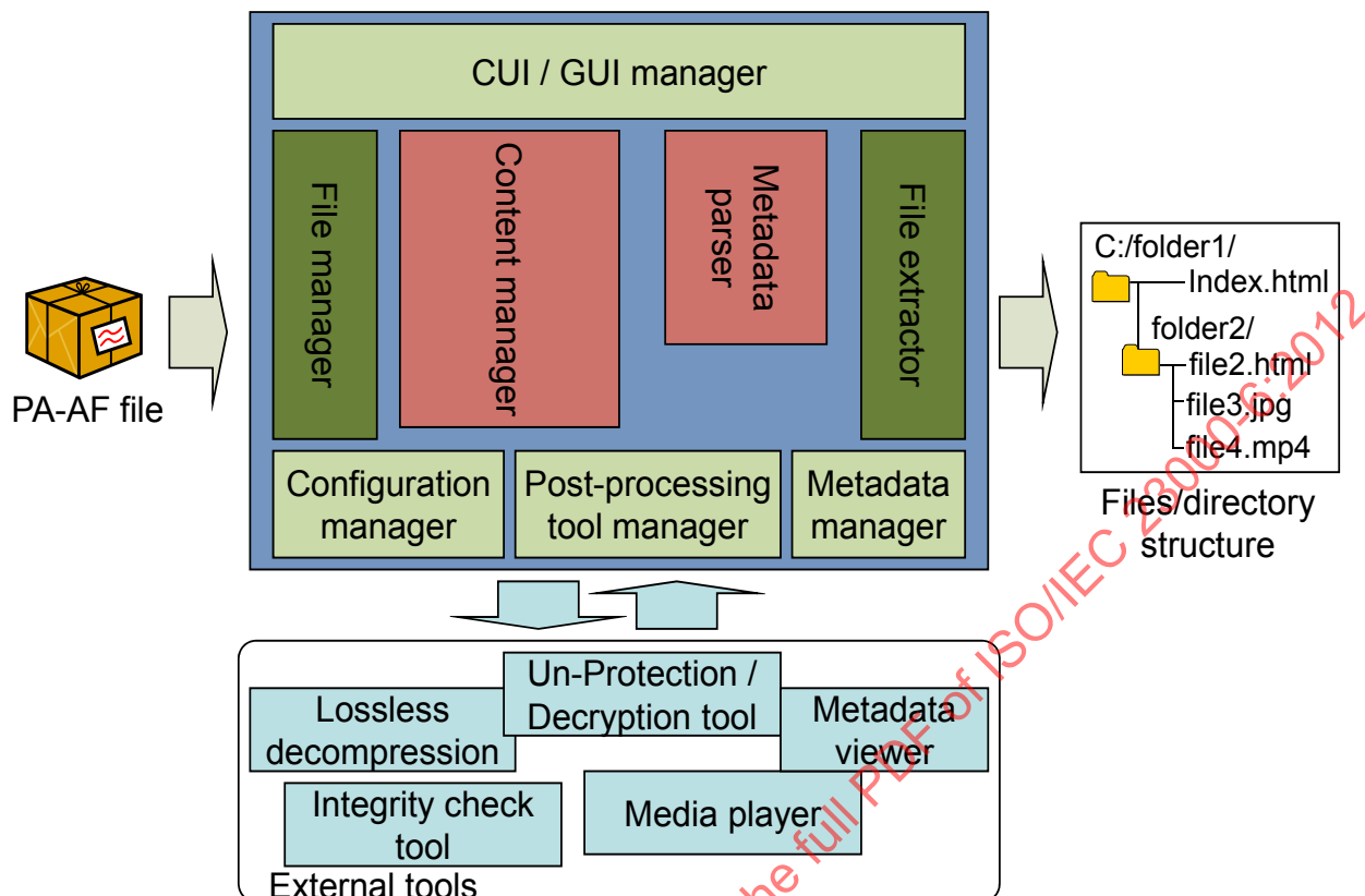
Figure 11 — PA-AF file extractor system architecture
