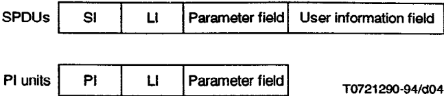
Figure 3 – Illustration of structure of SPDUs and PI units
