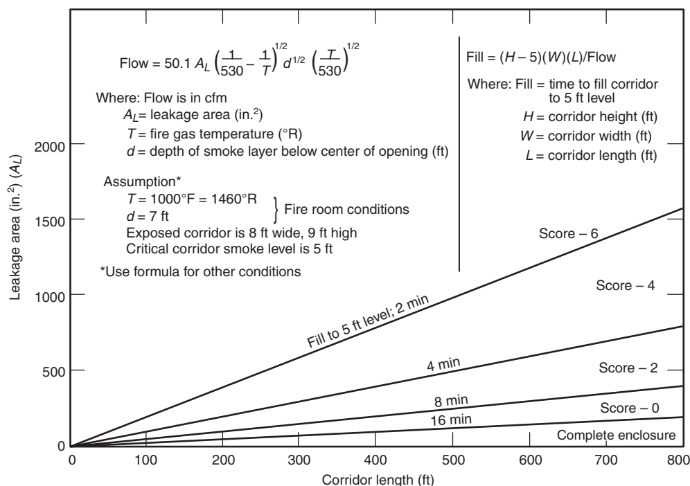
FIGURE 8.5.11.1.2 Approximate Time to Smoke Impact.
