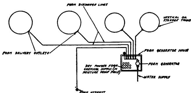
Fig. A-132(a)(1). Typical chemical foam generator system layout of the single powder type.
