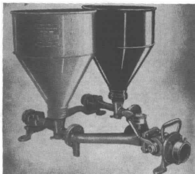
Fig. A-132(a)(5). Dual hopper chemical foam generator of the two powder type.
