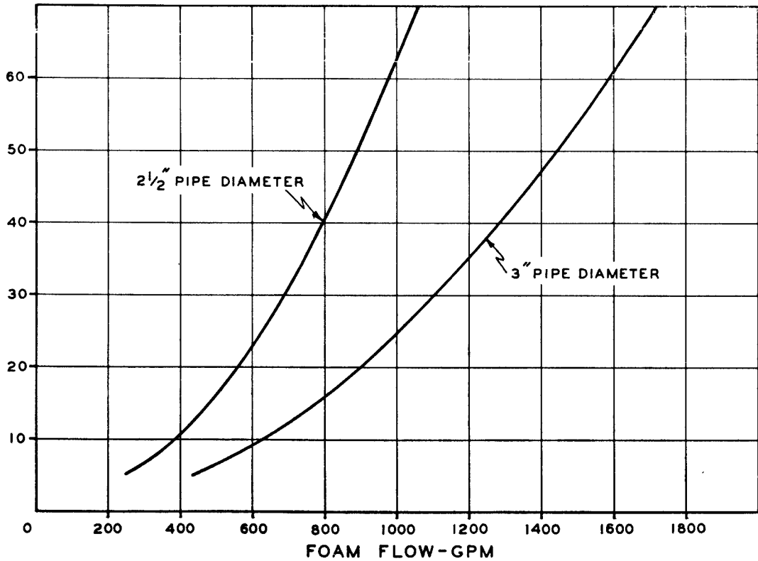
FRICTION LOSSES — PSI PER 100 FT. OF PIPE Fig. A-3561A
