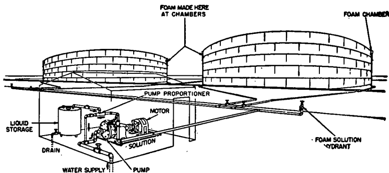
Fig. A-170. Schematic arrangement of air foam protection for storage tanks.
