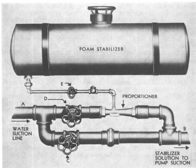
Fig. A-115. Pump Suction Proportioner. To install: connect A to water suction line, connect B to suction side of pump. To operate foam system: close valve C, open valves D and E. To discharge plain water: close valves D and E, open valve C.
