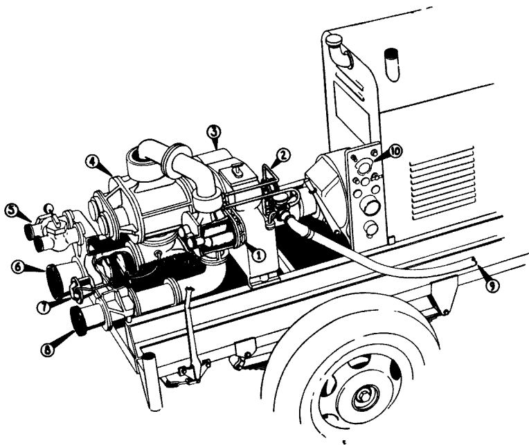
Fig. A-122(c). Air Foam Pump.
