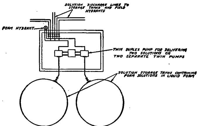
Fig. A-132(b)(2). Typical two solution (acid and basic) chemical foam system layout. Discharge line layout similar to that for two powder type shown in A-132(a)(2).
