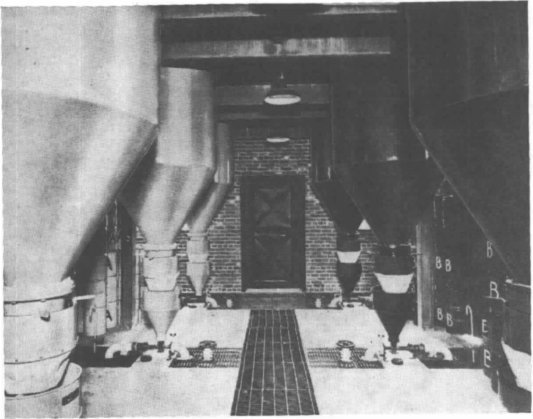
Fig. A-132(a)(3). Dual Powder Generator System with Powder in Bins.
