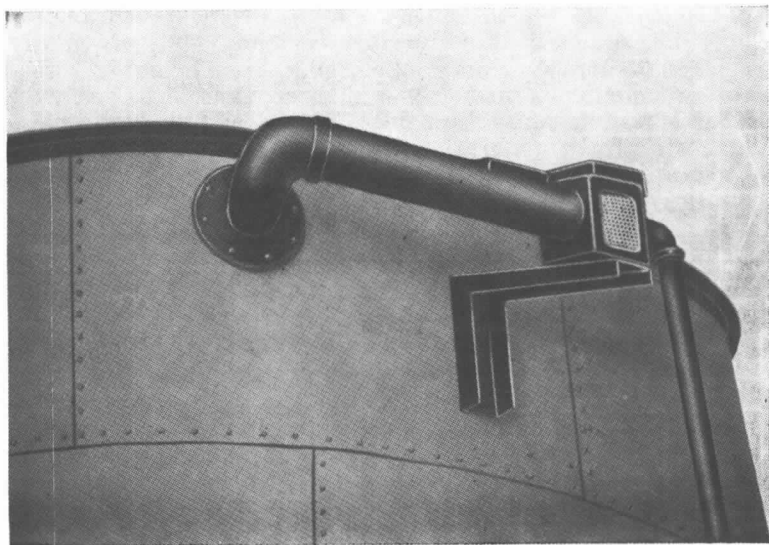
Fig. A-342A. Air Foam Maker in Horizontal Position at Top of Storage Tank.
