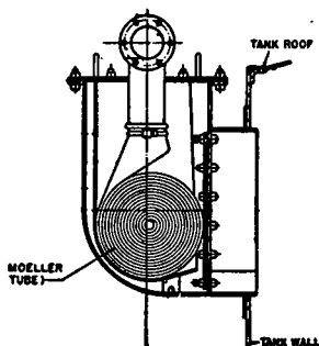
Fig. A-302A. Cross-section Moeller Tube Chamber. Tube is designed to unroll and fall to oil level. Foam flows through interstices in tube.
