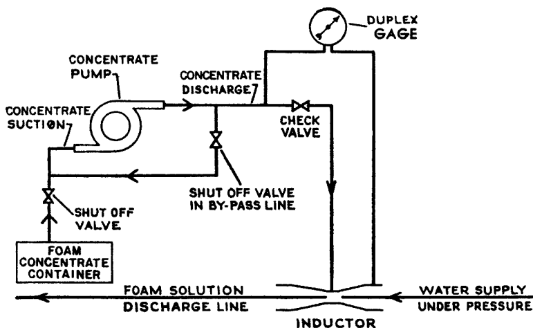
Fig. A-121(d). Metered Proportioning.
