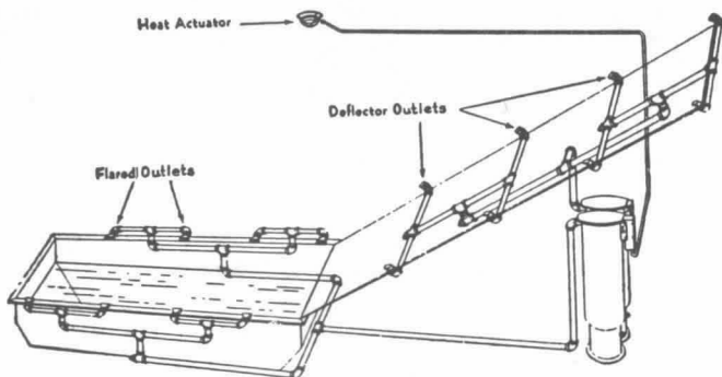
Fig. A-132(b)(1). An automatic chemical foam system of the stationary unit type protecting a dip tank and drain board.
