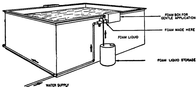
Fig. A-122(a)(1). Schematic diagram showing protection of dip tanks with air foam system. Foam liquid concentrate storage in vessel beside dip tank.
