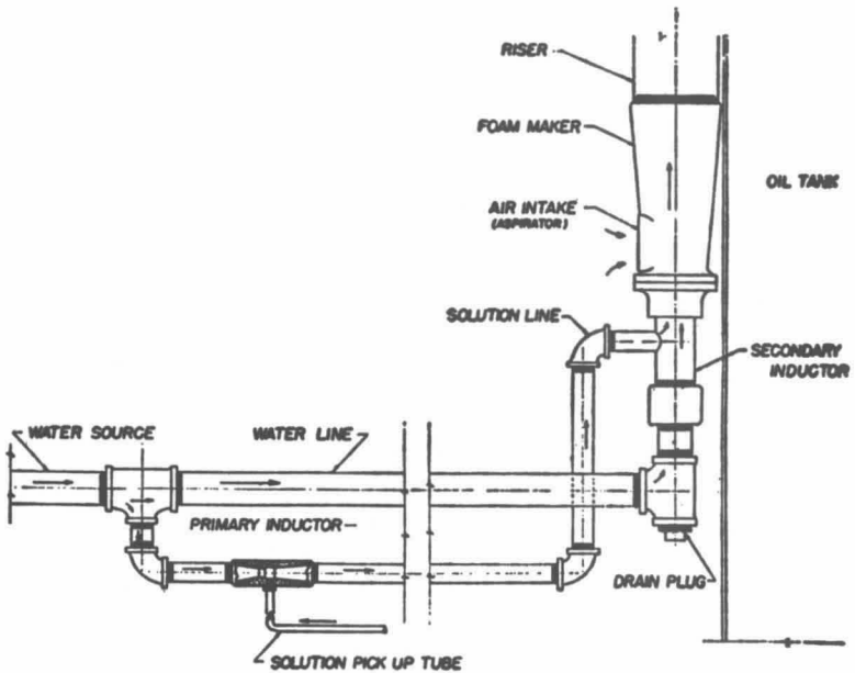
Fig. A-121(b)(2). Air Foam Auto-induction System. Solution pick-up tube picks up concentrate from its container.
