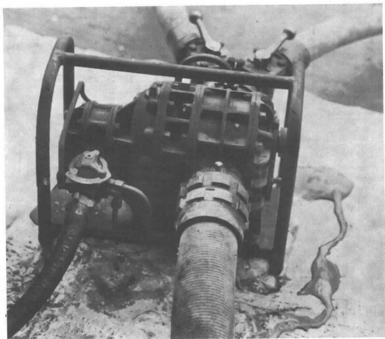
Fig. A-121(f). Coupled Water Motor Pump Proportioner.
