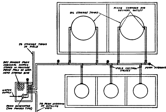
Fig. A-132(a)(2). Typical chemical foam generator system layout of the two powder type.
