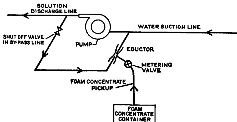
Fig. A-121(c). Around-the-Pump Proportioner.
