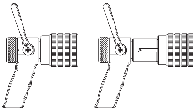
FIGURE 5.3.1.2.1(e) Combination Nozzle with Retractable Sleeve.
