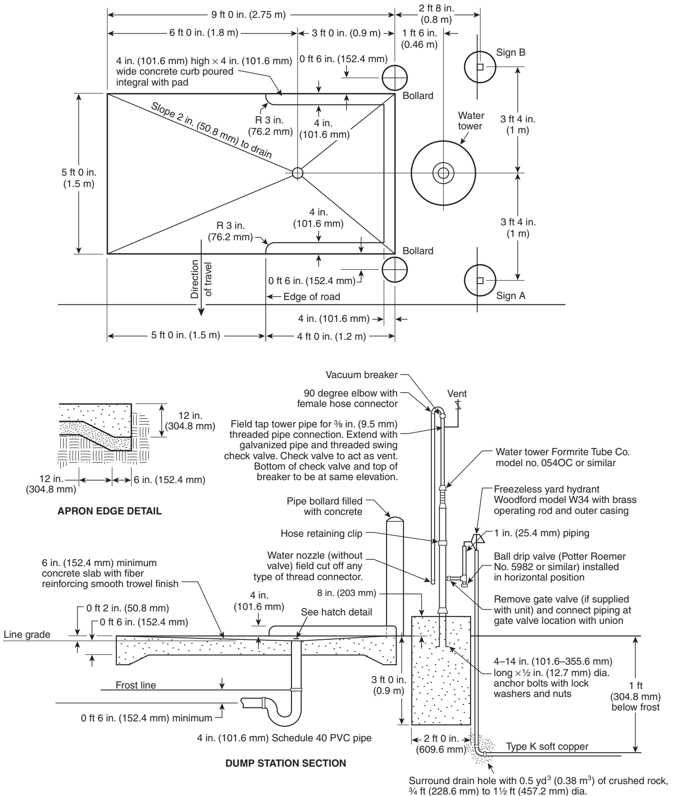
FIGURE B.1(h) One Optional Arrangement for a Sanitary Disposal Station on a Recreational Vehicle Park or Campground.
