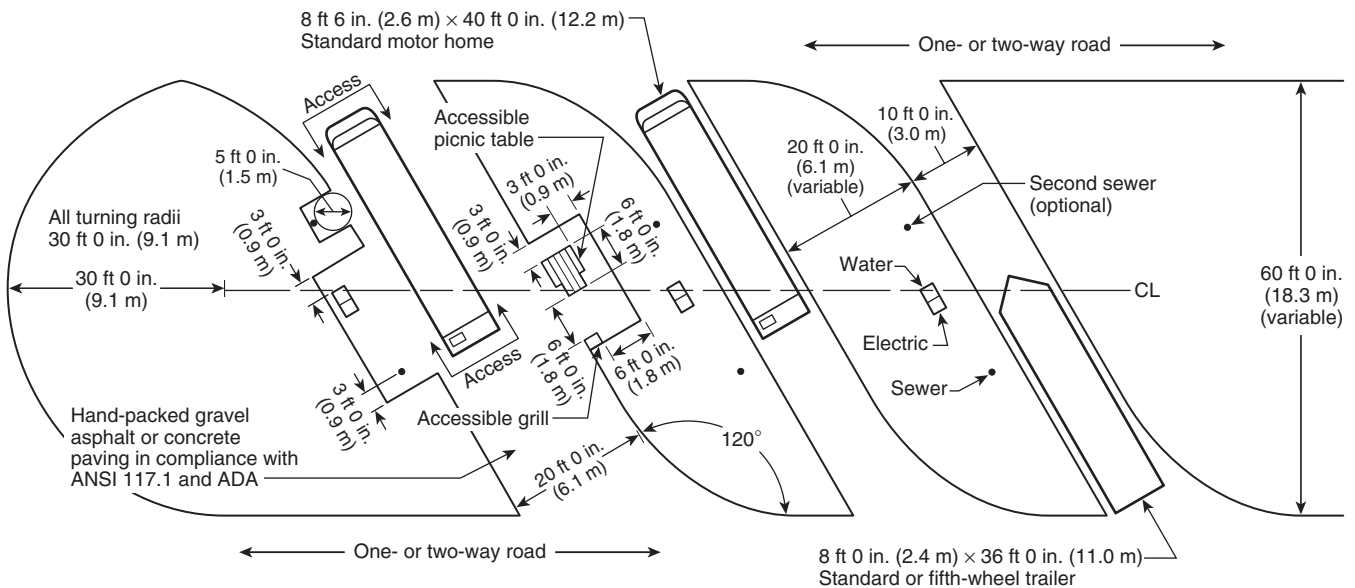
FIGURE B.1(d) One Optional Arrangement for a Recreational Vehicle Park or Campground for a Handicapped-Accessible Standard Pull-Through Site.
