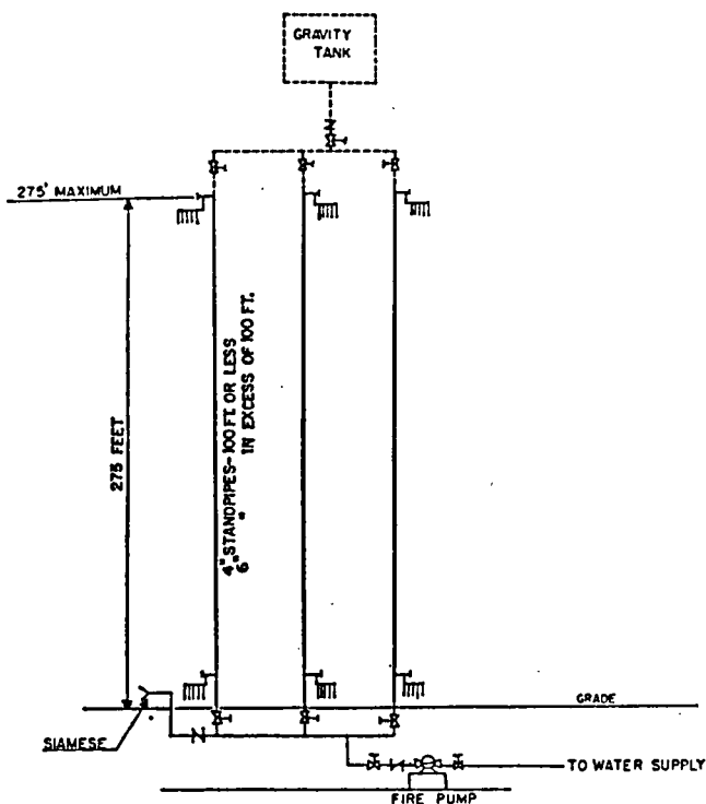
Figure 21-1. Single zone system.
