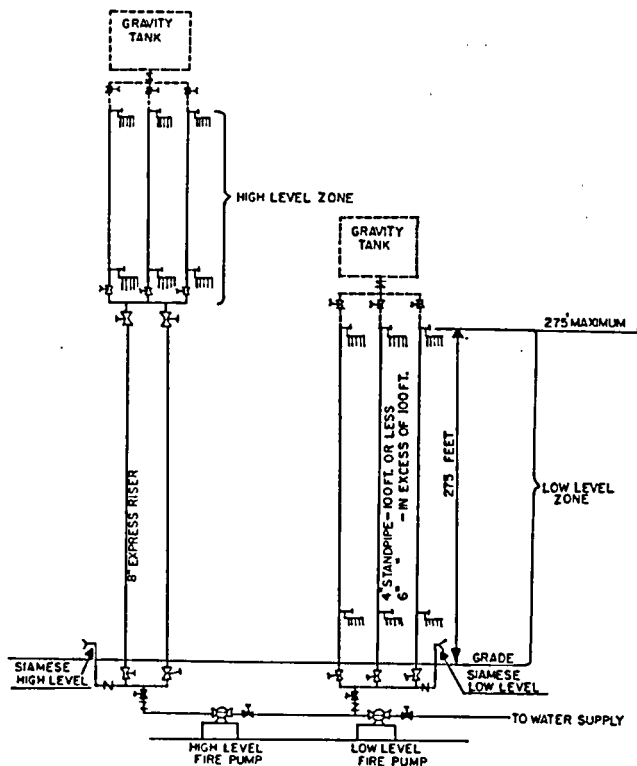
Figure 21-2. Two zone system.
