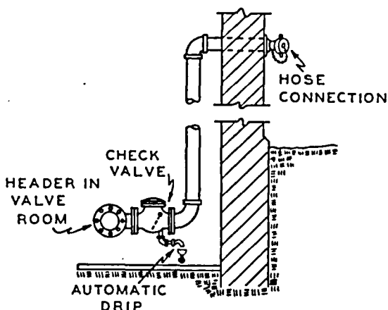
Figure 56. Fire department connection.
