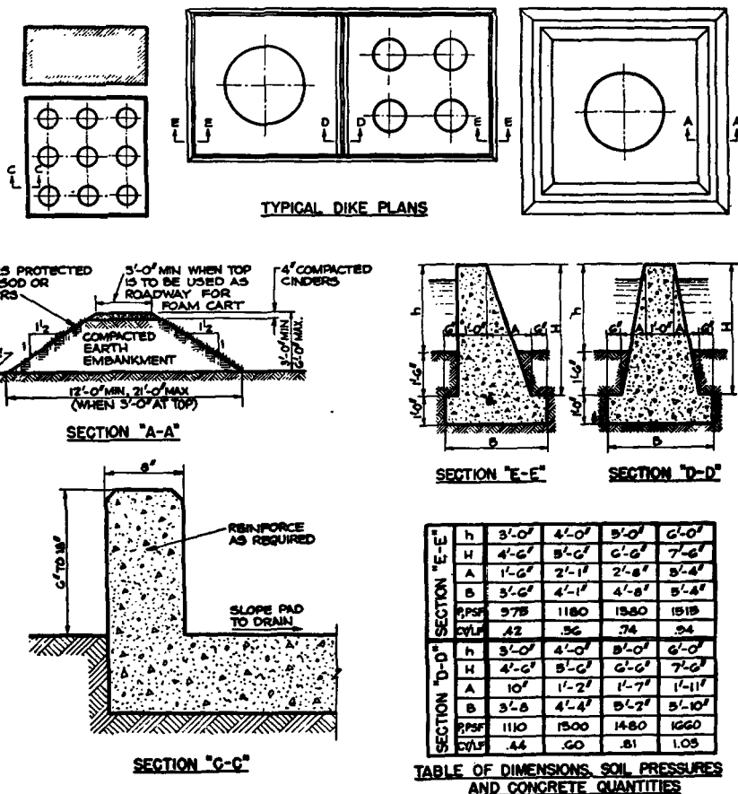
FIG. 4 STANDARD DIKES FOR FIELD STORAGE TANKS
