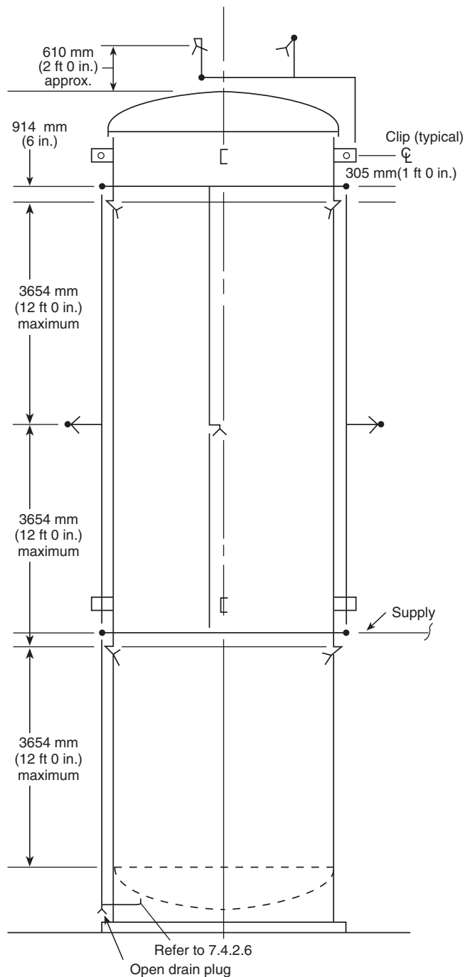
FIGURE A.7.4.2.2 Typical vertical tank with skirt protection.
