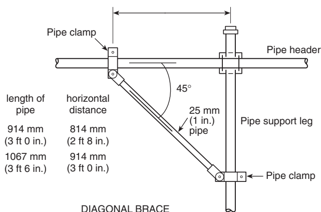
DIAGONAL BRACE
