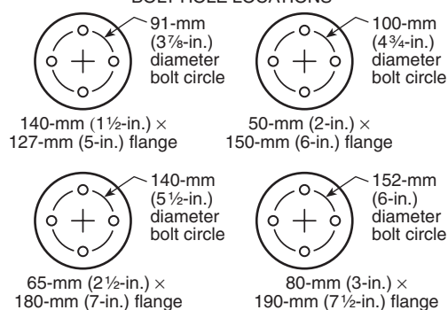
FIGURE A.6.3.2.4 Support leg footings.
