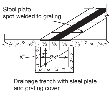
FIGURE A.4.4.4 Drainage trench detail.
