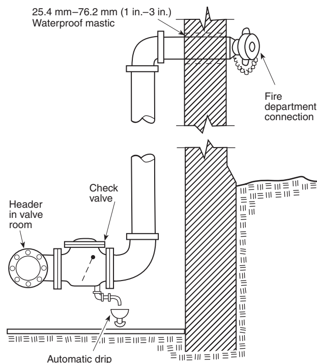
FIGURE A.6.4.3.1 Fire department connection.
