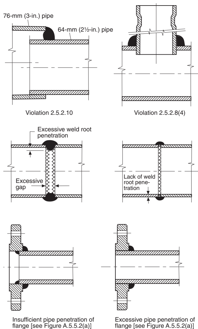
FIGURE A.5.5.2(b) Unacceptable weld joints.
