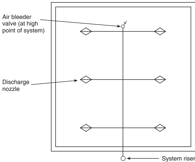
FIGURE A.12.3.1.2 Ultra high-speed area application for a small room.
