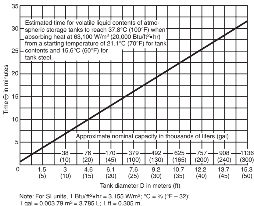
FIGURE A.7.4.2(a) Time-temperature curve.
