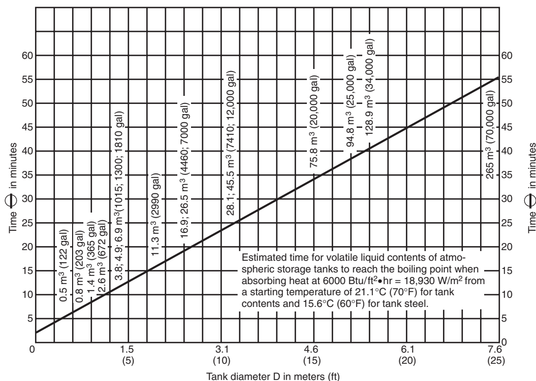
FIGURE A.7.4.2(b) Time-temperature curve.
