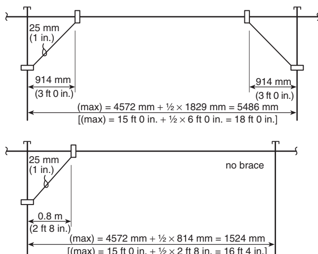
FIGURE A.6.3.2.2 Sway/support brace.
