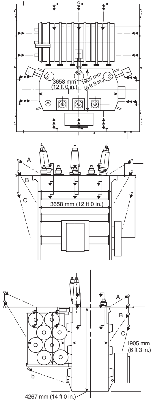
FIGURE A.7.4.4.1 Typical transformer layout.
