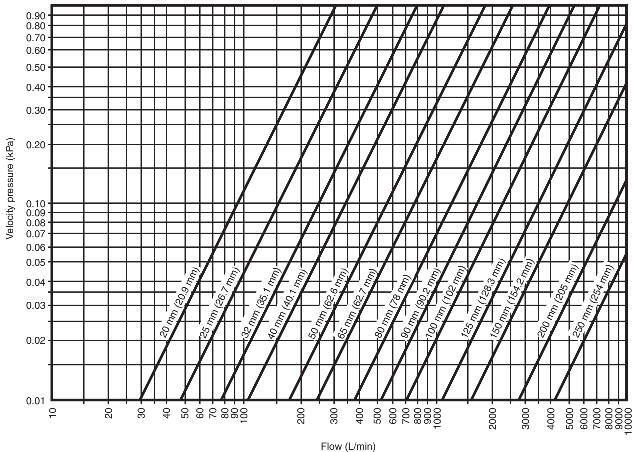
FIGURE A.8.5.1.2(a) Metric units. Graph for the determination of velocity pressure.
