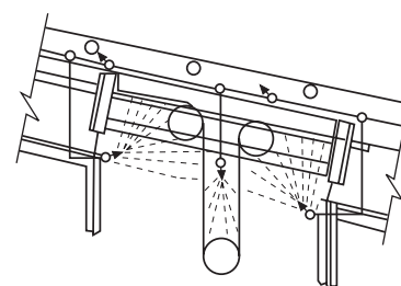
Elevation of typical take-up roller protection
