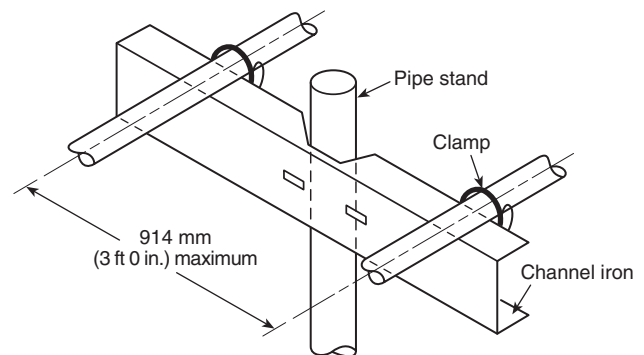
FIGURE A.6.3.2.2.5(d) Multiple pipes supported by one pipe stand.
