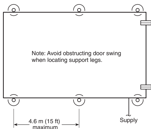
FIGURE A.6.3.2.1 Typical arrangement of support legs for pipe stands.
