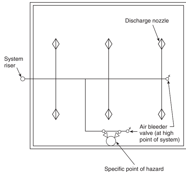
FIGURE A.12.3.1.3 Ultra high-speed dual application system.
