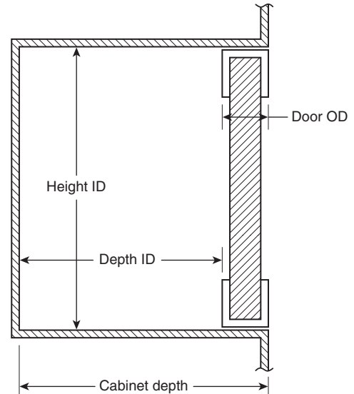
FIGURE A.6.16(b) Measurements of Interior Cabinets with Hinged Doors.
