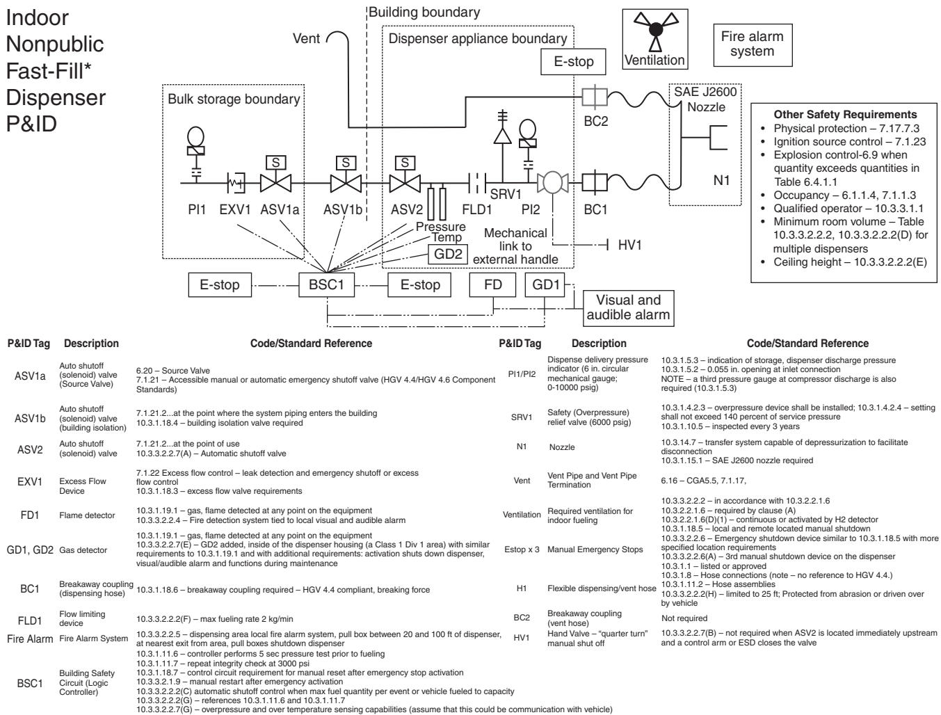
FIGURE A.10.5.3.2.2 Indoor Nonpublic Fast-Fill Dispenser P & ID.
