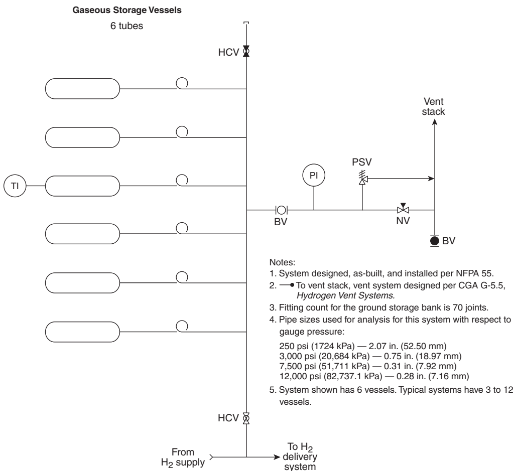
▲ FIGURE A.3.3.232.2(c) Typical Bulk Compressed Gaseous Storage System. [55:Figure A.3.3.95.9.1(c)]
