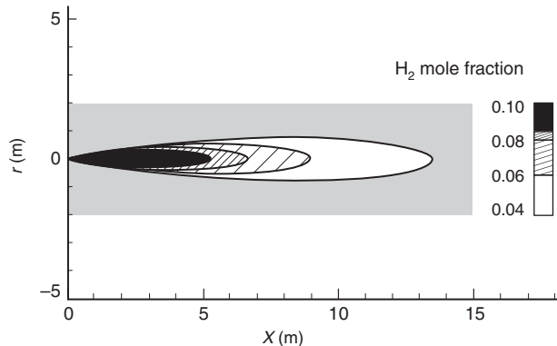
FIGURE E.4.1(d) Simulations of Concentration Decay of an Unignited Hydrogen Jet with a Diameter of 3.175 mm ( \frac{1}{8} in.) and a Tank Pressure of 207.85 bar (3000 psig). Contour lines correspond to mole fraction levels shown in the color legend.
