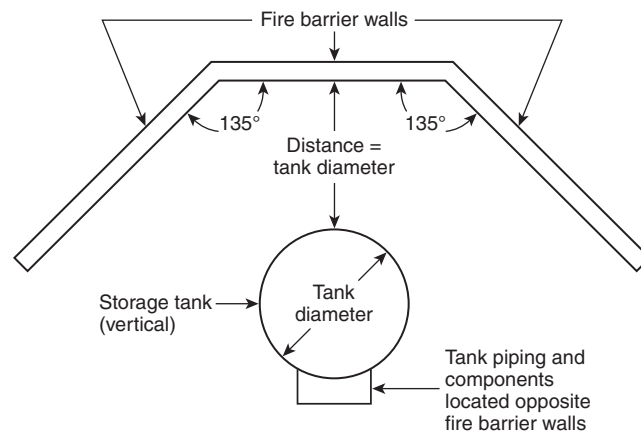
FIGURE A.8.3.2.3.1.6(A)(2)(c)(a) Schematic of Three-Sided Fire Barrier Wall Enclosure for a Vertical Hydrogen Storage System. [55:Figure A.11.3.2.2.5.2(a)]
