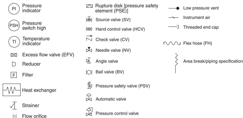
▲ FIGURE A.3.3.232.2(a) Symbol Legend for Figure A.3.3.263.10.2.1(b) through Figure A.3.3.263.10.2.1(f). [55:Figure 3.3.95.9.1(a)]
