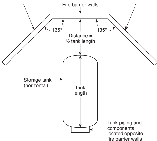
▲ FIGURE A.8.3.2.3.1.6(A)(2)(c)(b) Schematic of Three-Sided Fire Barrier Wall Enclosure for a Horizontal Hydrogen Storage System. [55:Figure A.11.3.2.2.5.2(b)]
