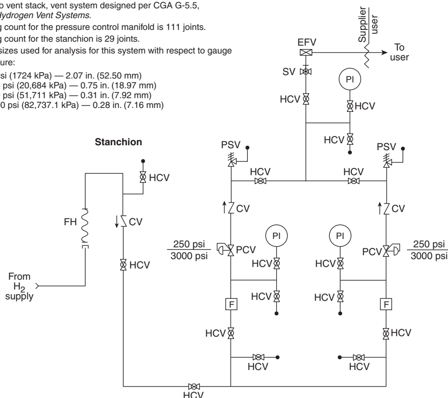
▲ FIGURE A.3.3.232.2(d) Typical Tube Trailer Discharge Stanchion and Pressure Control Manifold. [55:Figure A.3.3.95.9.1(d)]
