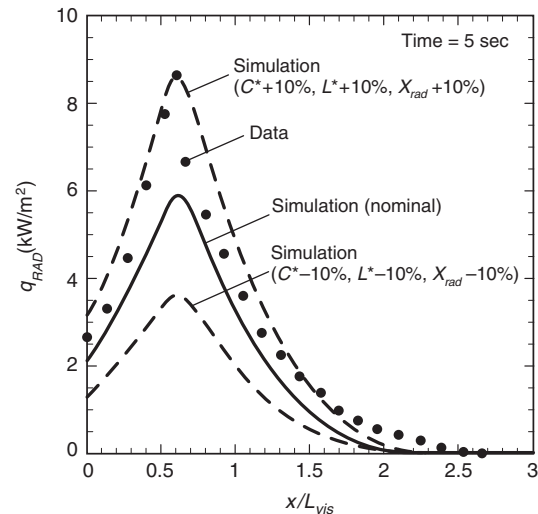
FIGURE E.3.1(b) Comparison of Simulation of Radiative Heat Flux from a Hydrogen Flame at a Radial Position of r = 1.83 \text{ m} with the Data at 5 Seconds into the Blow-Down.
