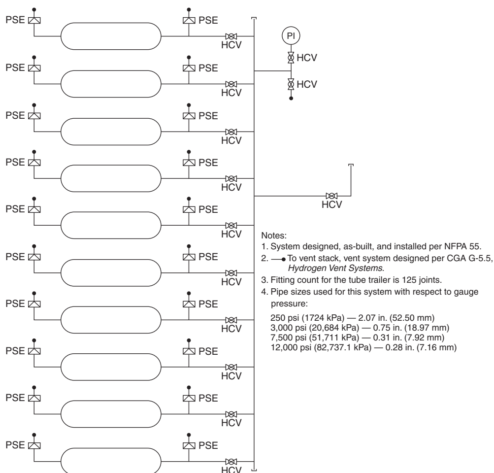
▲ FIGURE A.3.3.232.2(b) Typical Tube Trailer. [55:Figure A.3.3.95.9.1(b)]
