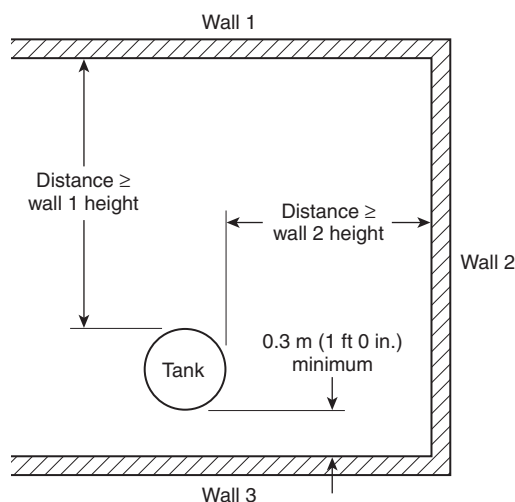
Δ FIGURE A.8.3.2.3.1.5(D)(1) Bulk Cryogenic System Located in a Courtyard. [55:Figure A.8.12.2.7.2.1]
