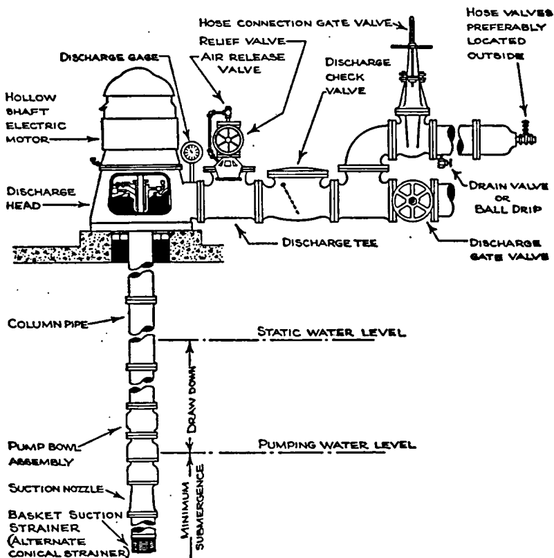
Fig. 201. Vertical Shaft Turbine-Type Pump Installation.
