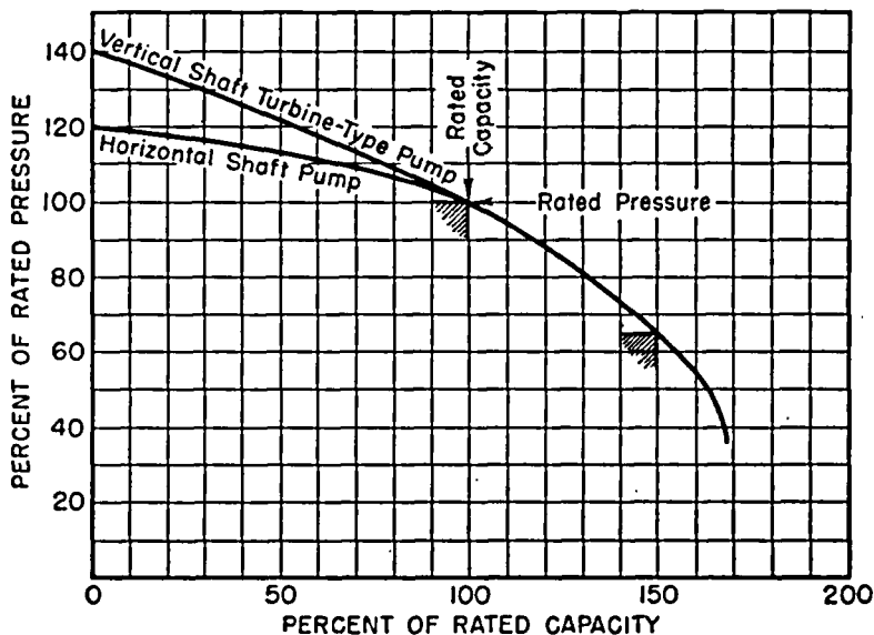
Fig. 13. Characteristic Curves.
