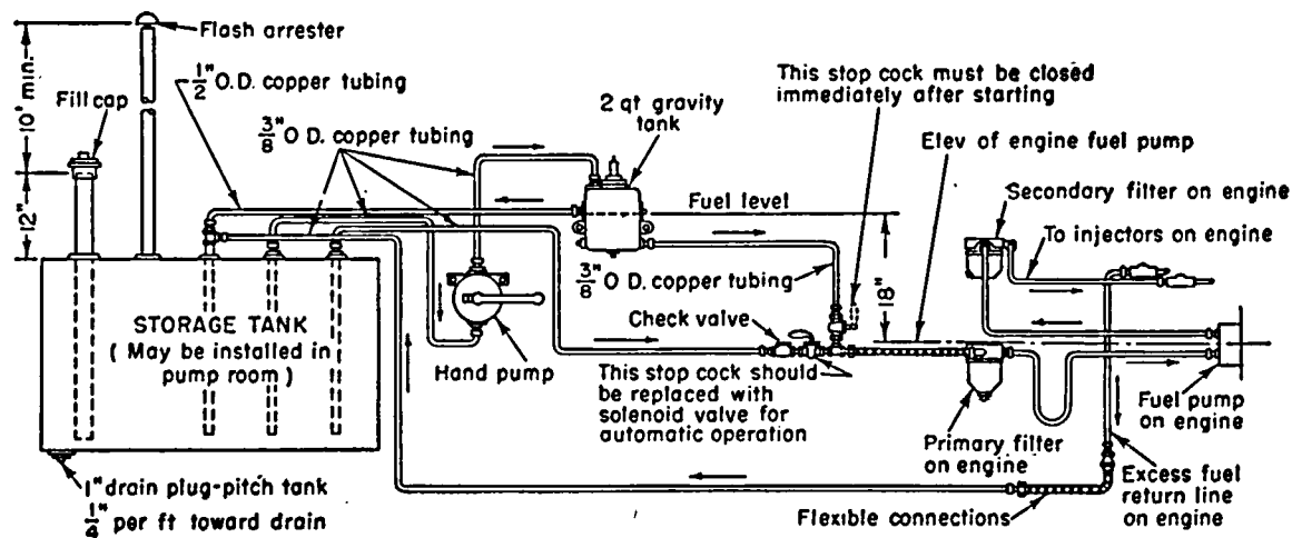
Fig. 606. Fuel System for Diesel Engine Driving Fire Pump.
